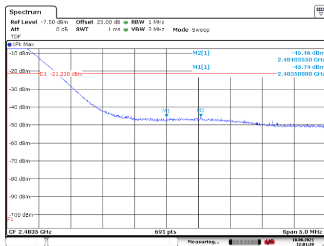
Figure 8.7-7: Conducted spurious emissions at band edge within restricted band, TX on High channel, Peak
