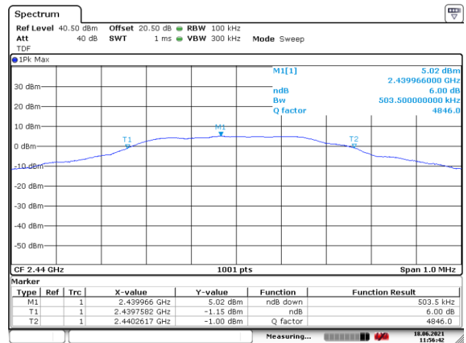
Figure 8.5-2: 6 dB bandwidth on BLE, Tx mid channel
