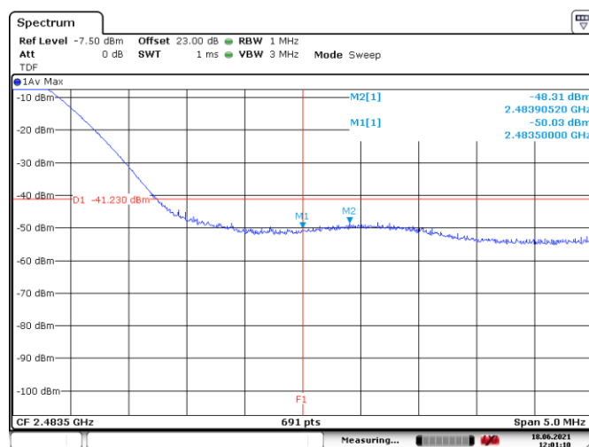
Figure 8.7-9: Conducted spurious emissions at band edge within restricted band, TX on High channel, average
