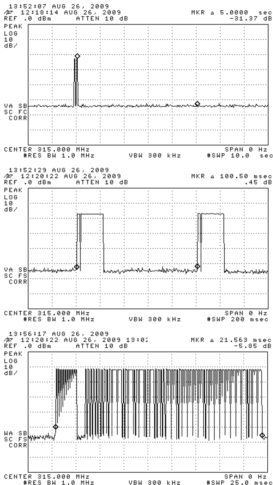
Figure 6.1(a). Transmission modulation characteristics. (top) complete transmission from single button press, (center) expanded transmission, (bottom) expanded word.
