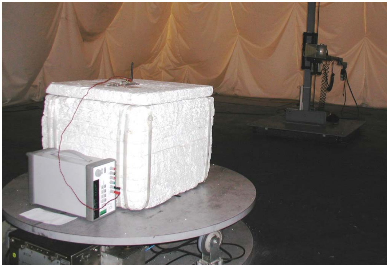
Photo 15: Test setup for radiated spurious emissions below 18GHz with EMCO 3115 horn antenna in vertical polarity and Elektronika AIM4M1 Module using 2dBi whip in vertical orientation
