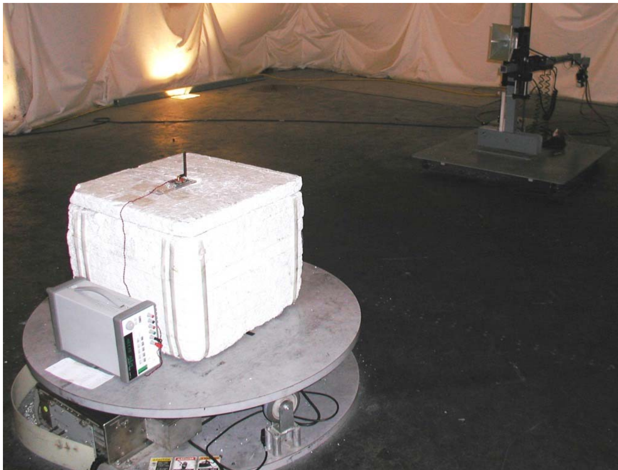
Photo 16: Test setup for radiated spurious emissions below 18GHz with EMCO 3115 horn antenna in horizontal polarity and Alektrona AIM4M1 Module using 2dBi whip in vertical orientation
