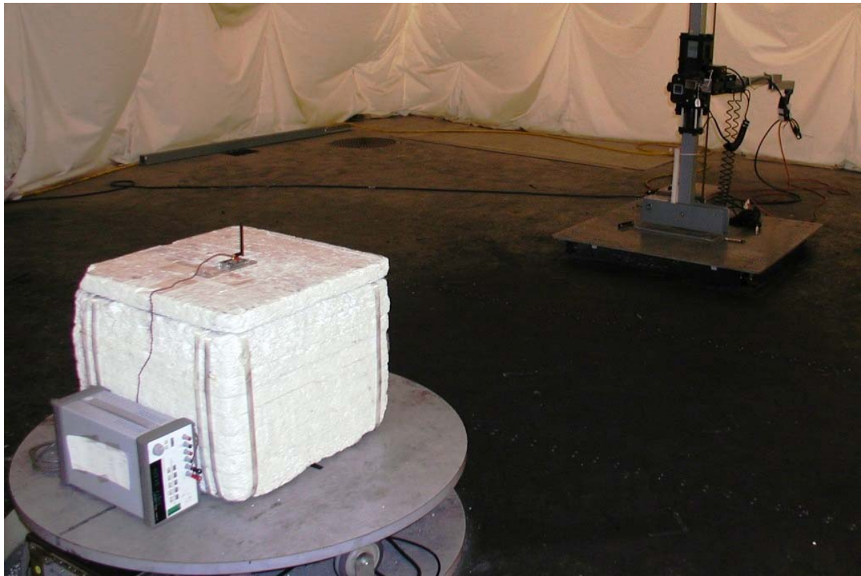
Photo 20: Test setup for radiated spurious emissions above 18GHz with AH Systems SAS-572 horn antenna in vertical polarity and Alektrona AIM4M1 Module using 2dBi whip in vertical orientation
