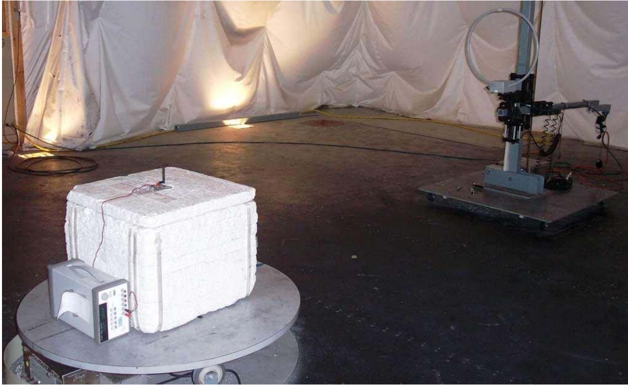
Photo 1: Test setup for radiated spurious between 9kHz and 30MHz with EMCO 6502 Loop Antenna shown and Alektrona AIM4M1 Module using 2dBi whip in vertical orientation
