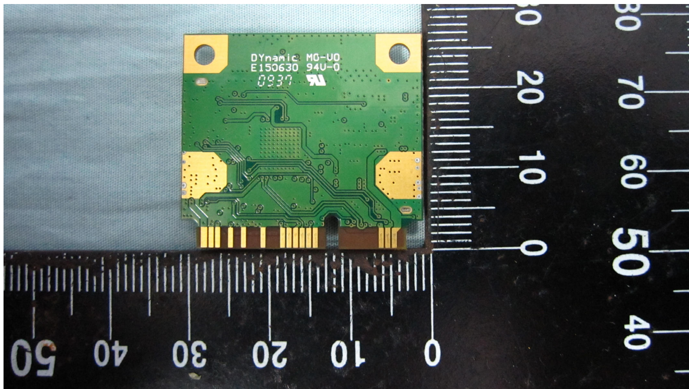
Inner View of WLAN Card
