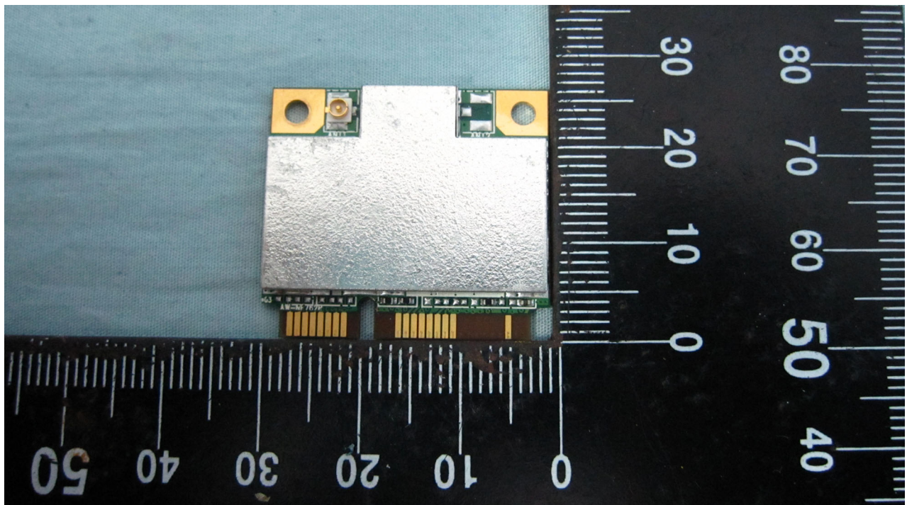
Rear View of WLAN Card
