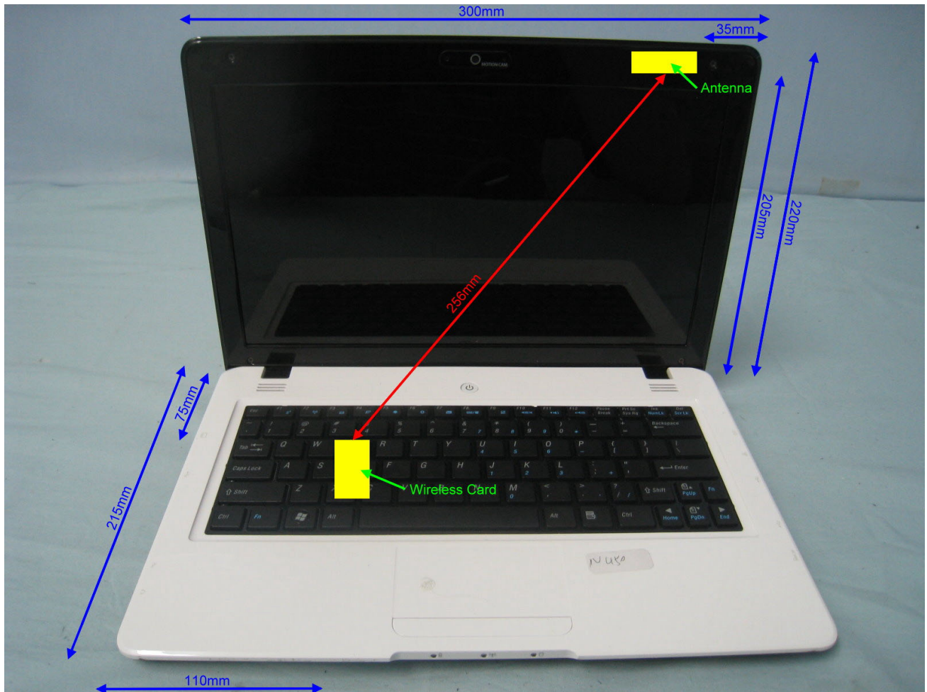
Antenna Location and EUT Dimension
