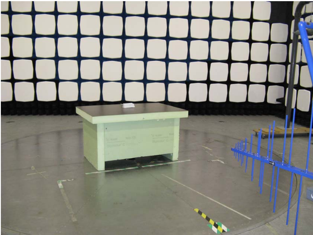
30 – 1000 MHz
