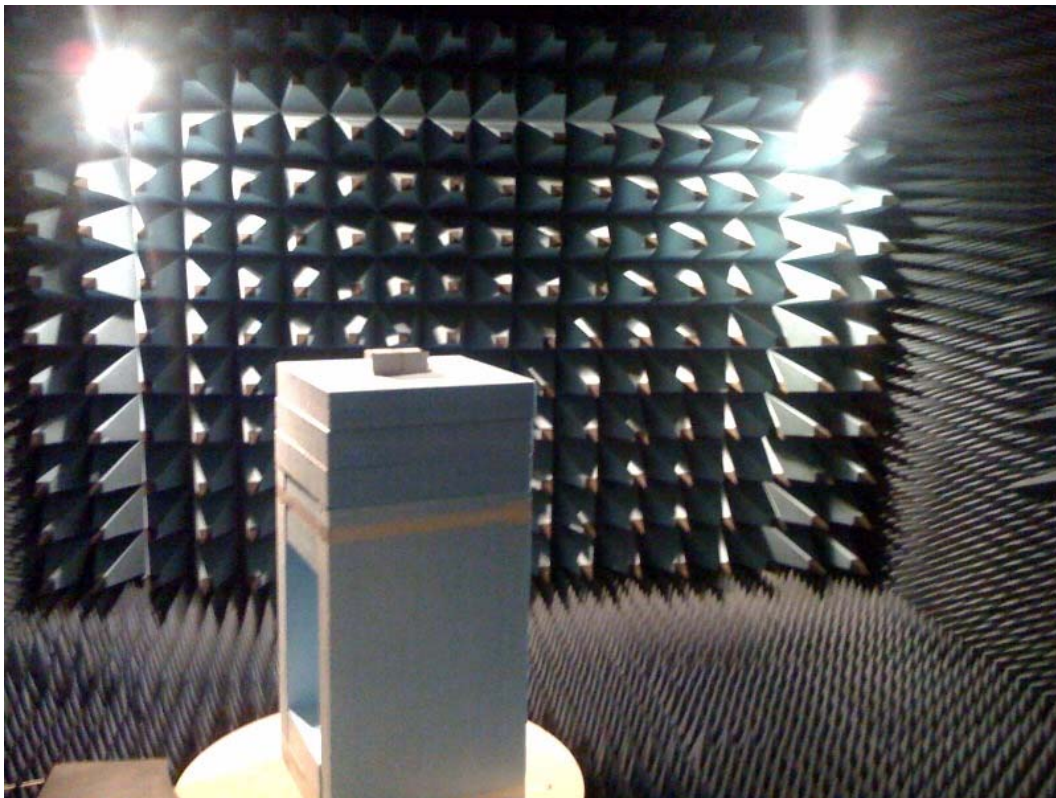
1 – 26 GHz
