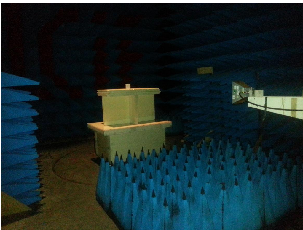
Radiated emissions measurements setup above 1GHz
