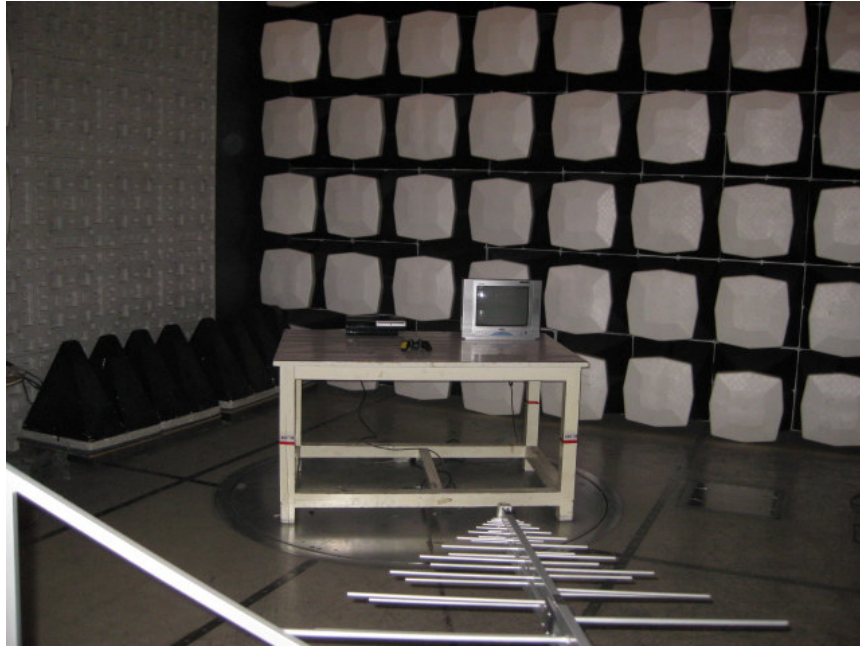
Radiated Emission
