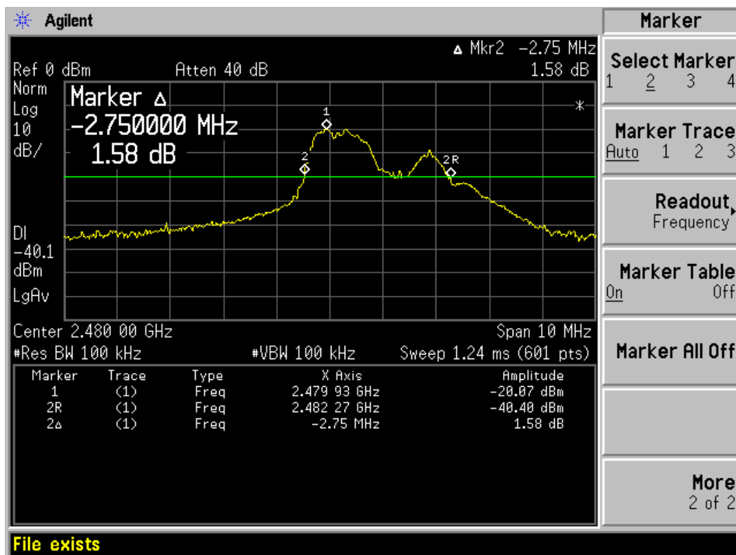
Channel 79_ 2480 MHz
