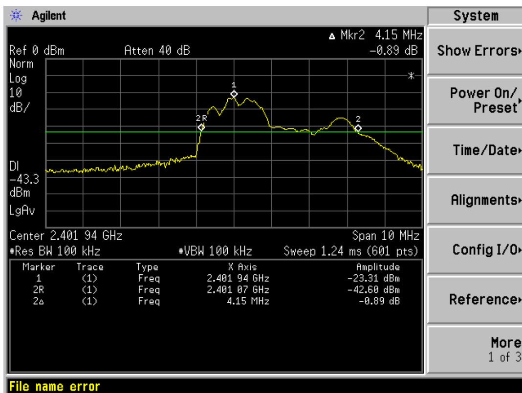
Channel 1_ 2402 MHz
