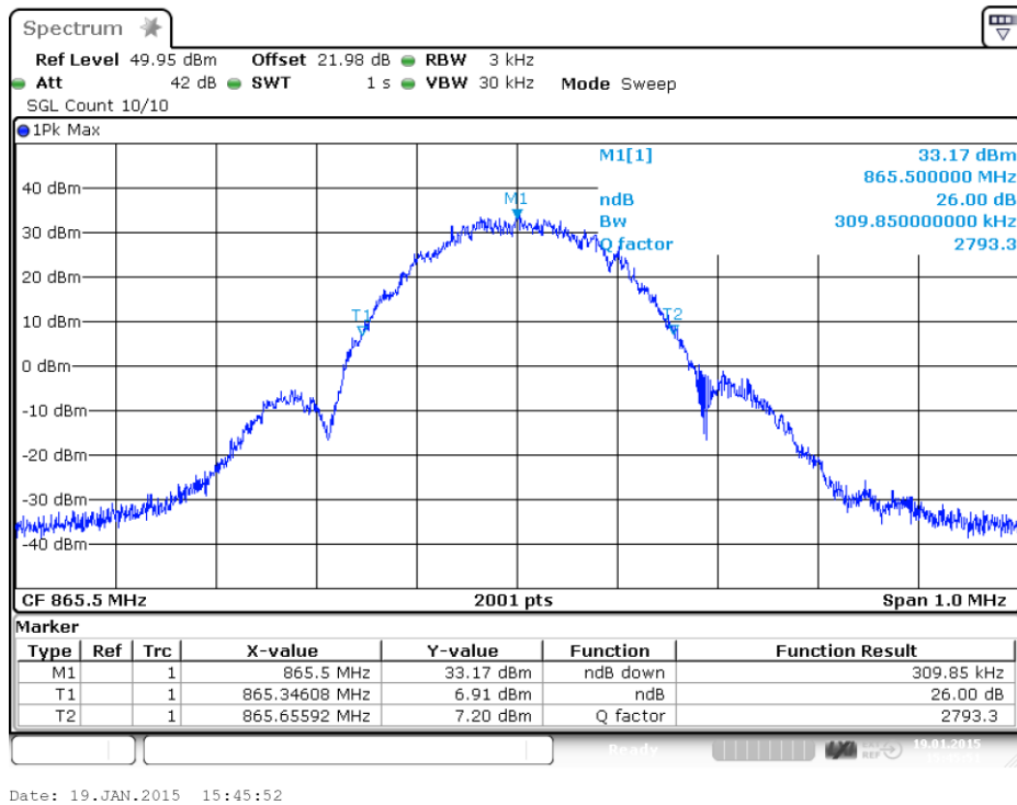
plot 6.3.2.2-#1 Occupied Bandwidth: $90.210, $2.1049; Test results; 26dB BW; EDGE Output
