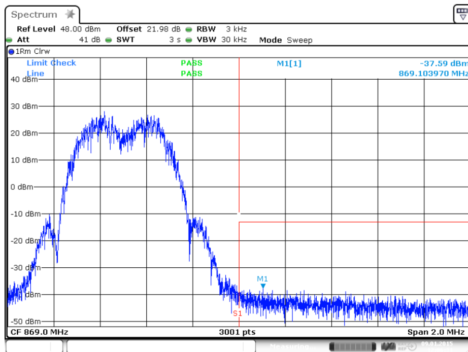
plot 8.3.1.2-#2 Intermodulation: §90.210, §2.1051; Test results; Downlink; EDGE Upper Band Edge
