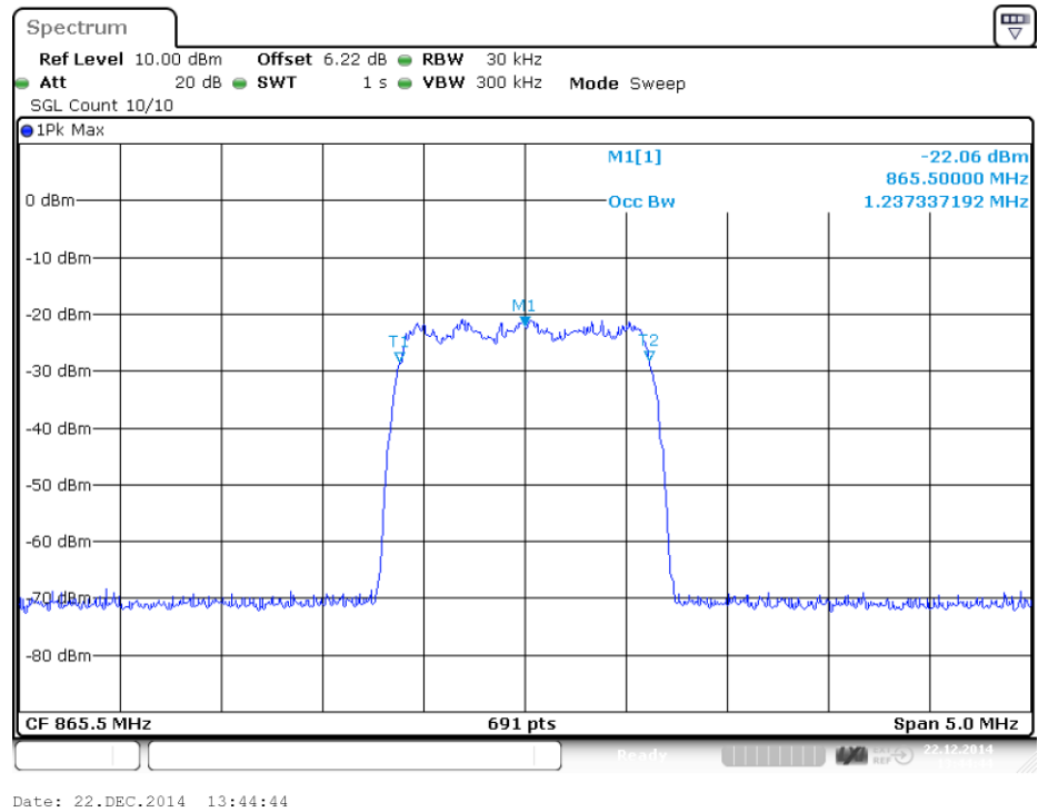
plot 6.3.1.3-#2 Occupied Bandwidth: $90.210, $2.1049; Test results; Downlink; CDMA Input
