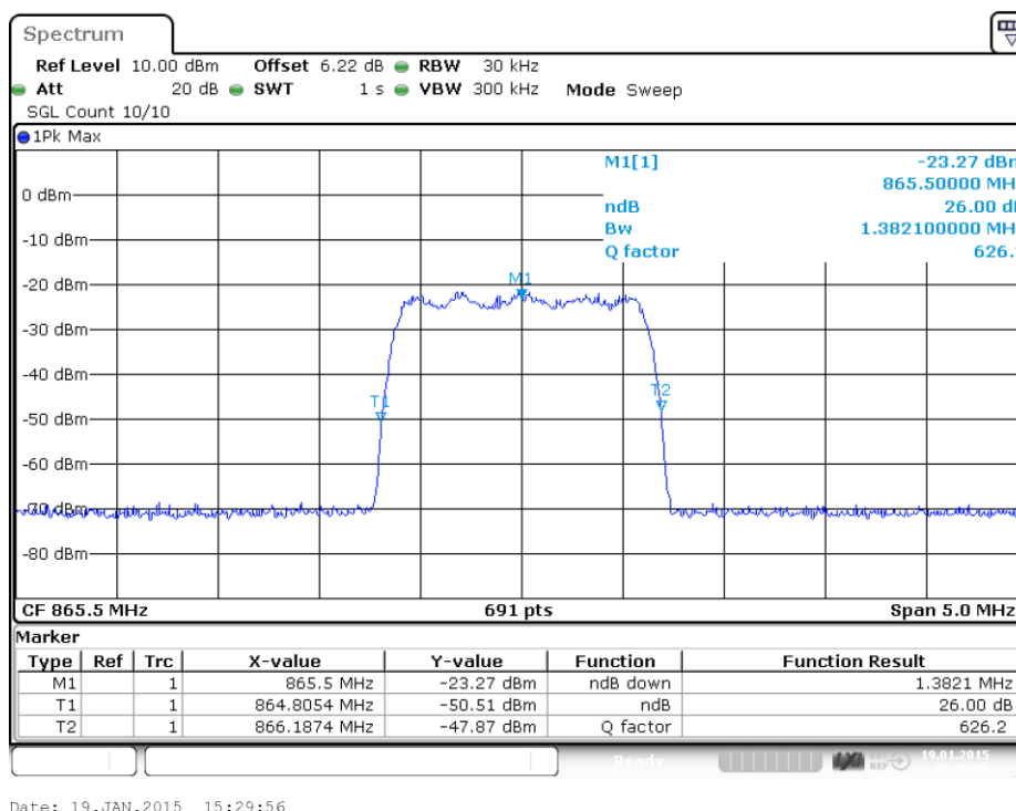
plot 6.3.2.3-#2 Occupied Bandwidth: $90.210, $2.1049; Test results; 26dB BW; CDMA Input
