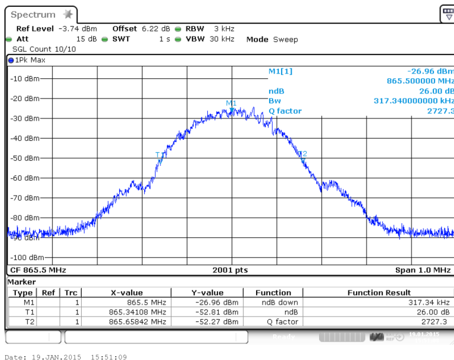
plot 6.3.2.1-#2 Occupied Bandwidth: $90.210, $2.1049; Test results; 26dB BW; GSM Input
