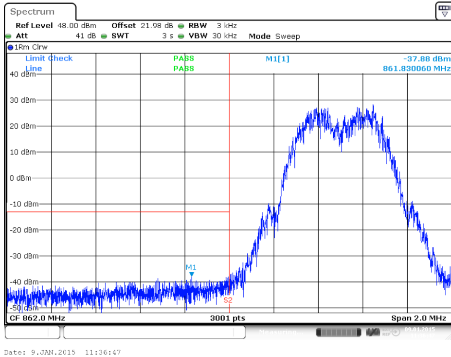
plot 8.3.1.1-#1 Intermodulation: §90.210, §2.1051; Test results; Downlink; GSM Lower Band Edge
