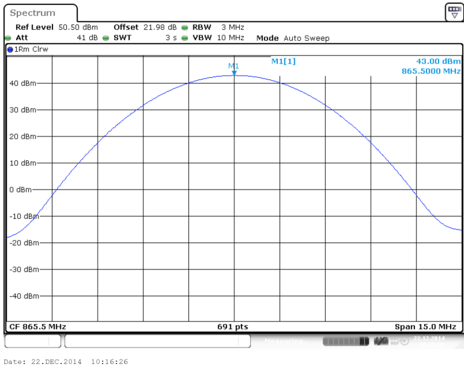
plot 5.3.1.3-#1 RF Power Out: §90.635, §2.1046; Test Results; Downlink; CDMA Middle
