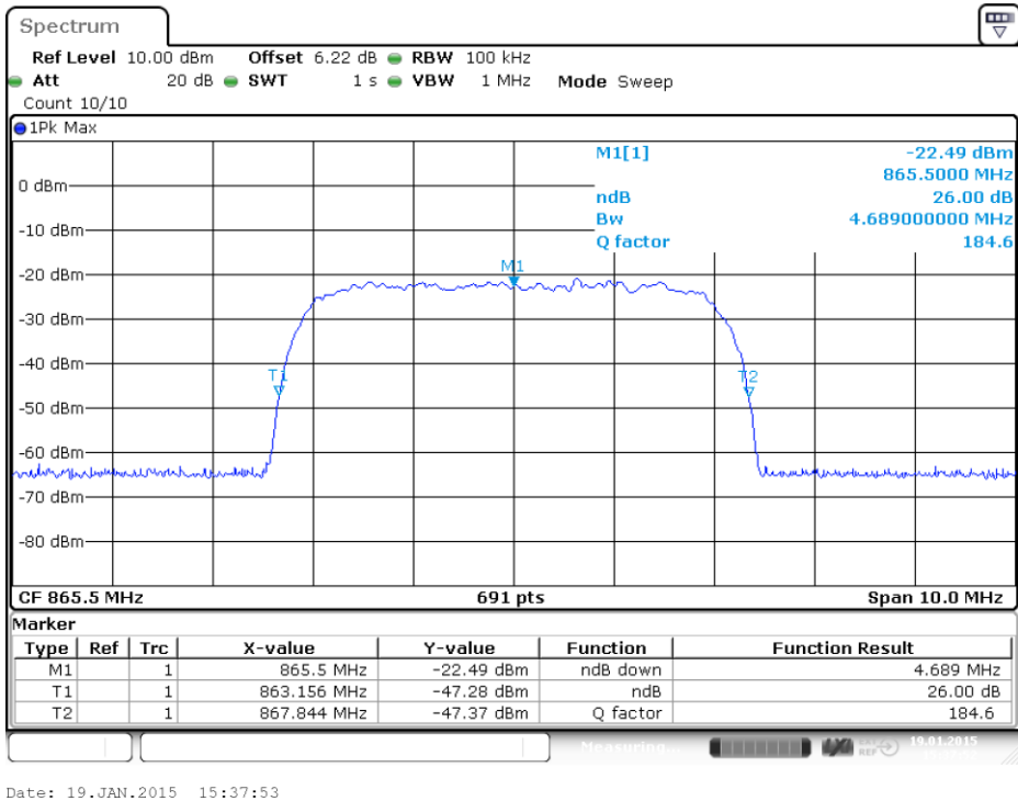
plot 6.3.2.4-#2 Occupied Bandwidth: §90.210, §2.1049; Test results; 26dB BW; WCDMA Input
