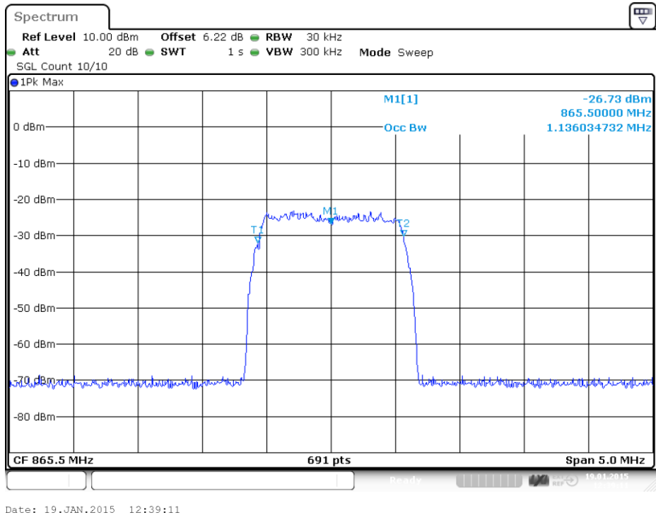
plot 6.3.1.5-#2 Occupied Bandwidth: $90.210, $2.1049; Test results; Downlink; LTE Input
