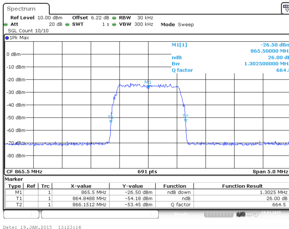
plot 6.3.2.5-#2 Occupied Bandwidth: §90.210, §2.1049; Test results; 26dB BW; LTE Input
