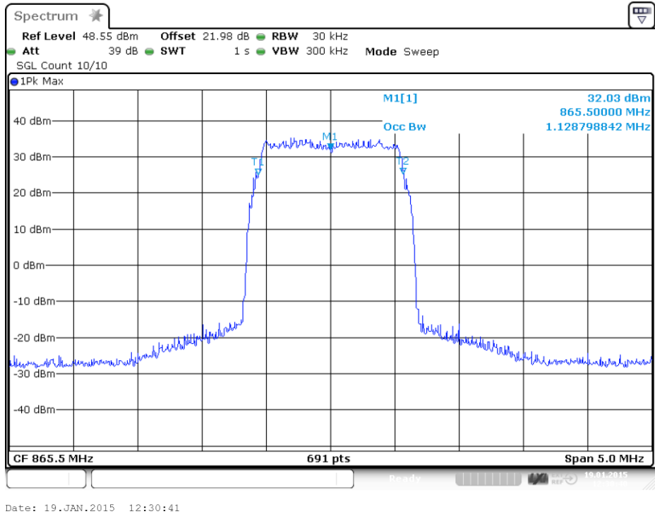
plot 6.3.1.5-#1 Occupied Bandwidth: $90.210, $2.1049; Test results; Downlink; LTE Output
