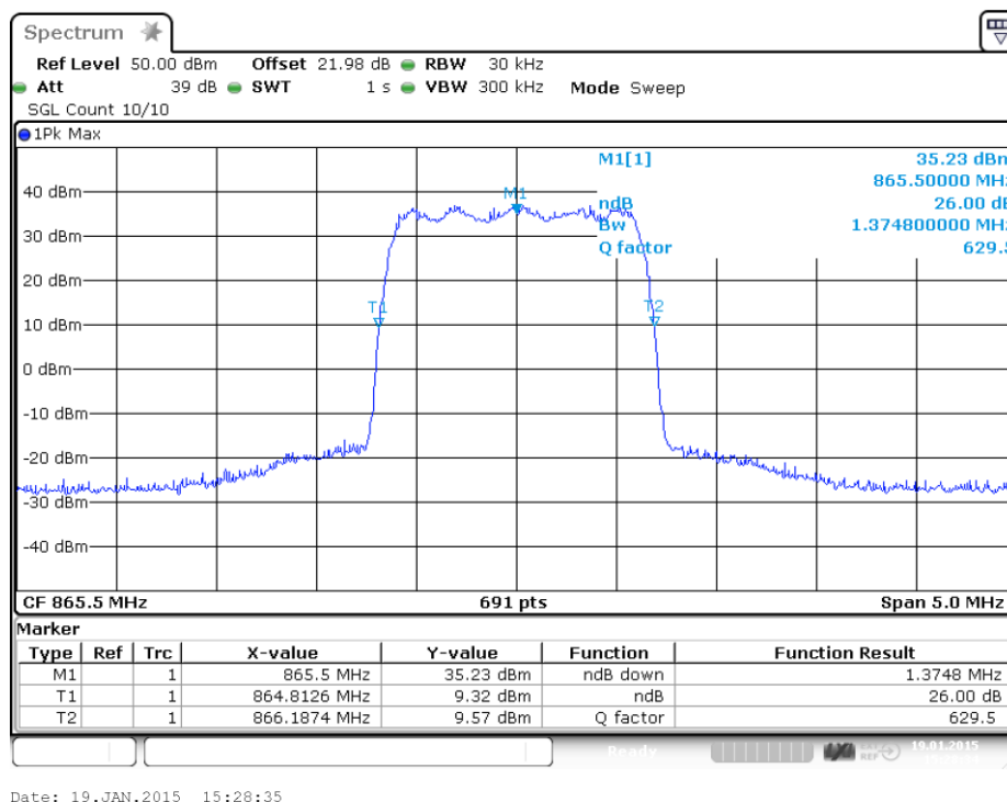
plot 6.3.2.3-#1 Occupied Bandwidth: $90.210, $2.1049; Test results; 26dB BW; CDMA Output
