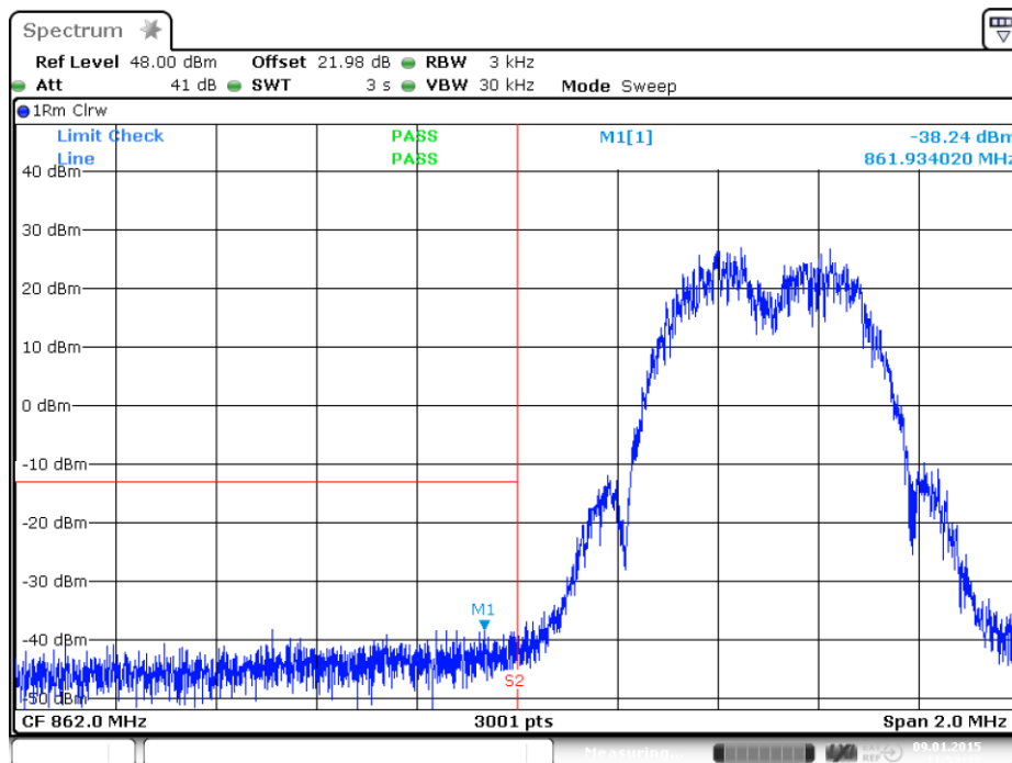
plot 8.3.1.2-#1 Intermodulation: §90.210, §2.1051; Test results; Downlink; EDGE Lower Band Edge
