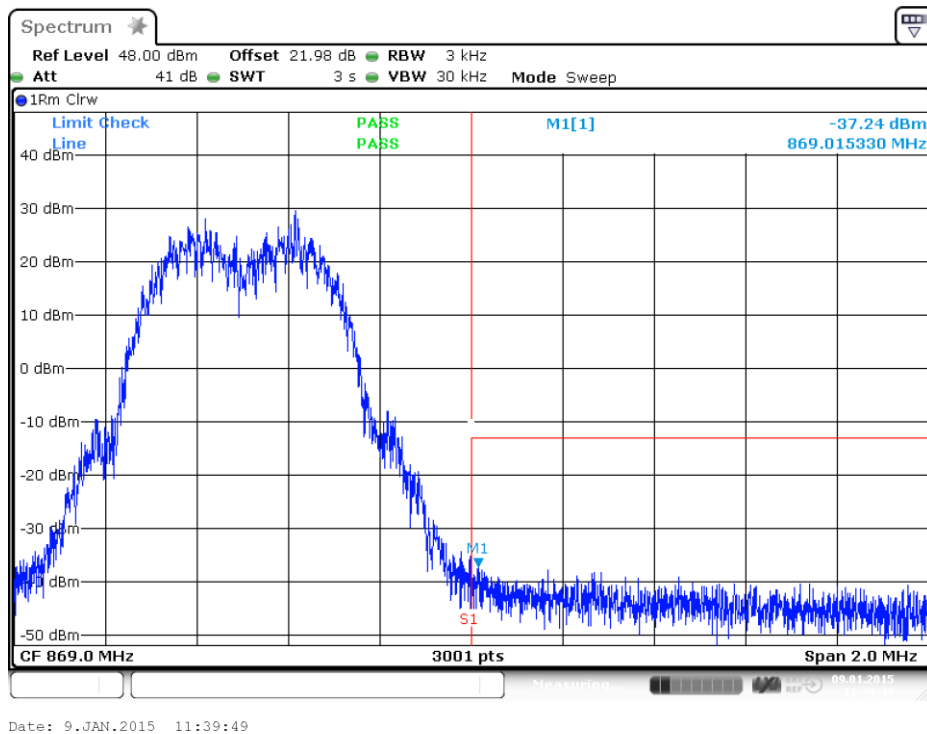
plot 8.3.1.1-#2 Intermodulation: §90.210, §2.1051; Test results; Downlink; GSM Upper Band Edge
