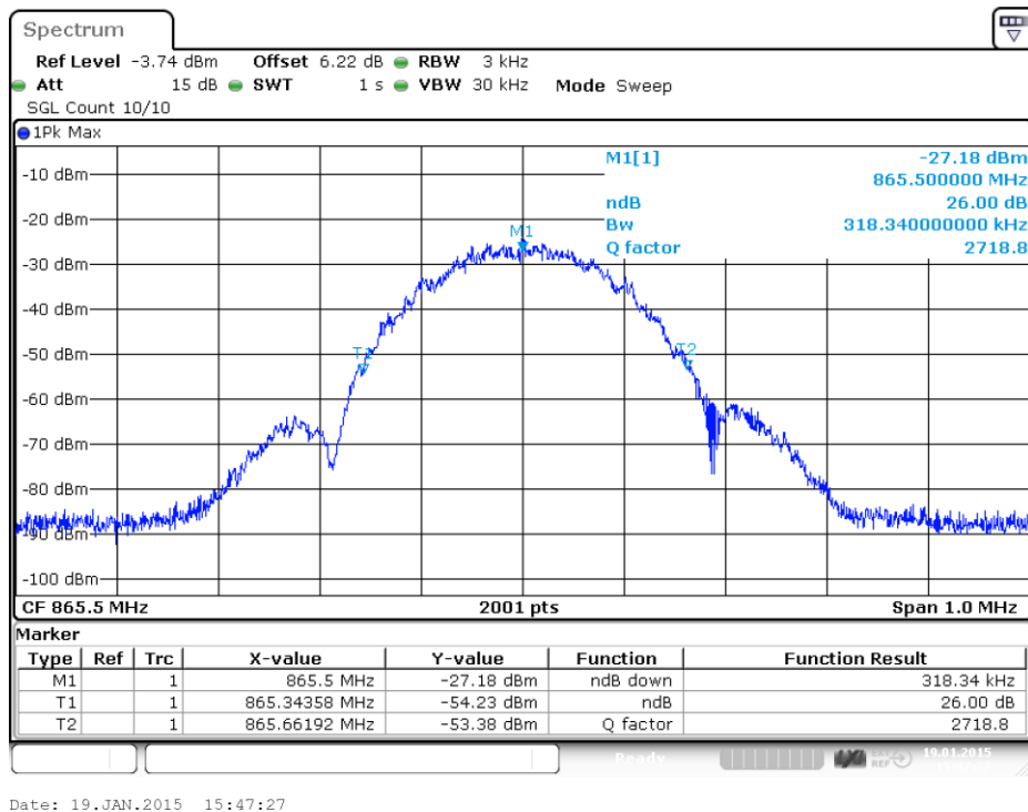
plot 6.3.2.2-#2 Occupied Bandwidth: $90.210, $2.1049; Test results; 26dB BW; EDGE Input
