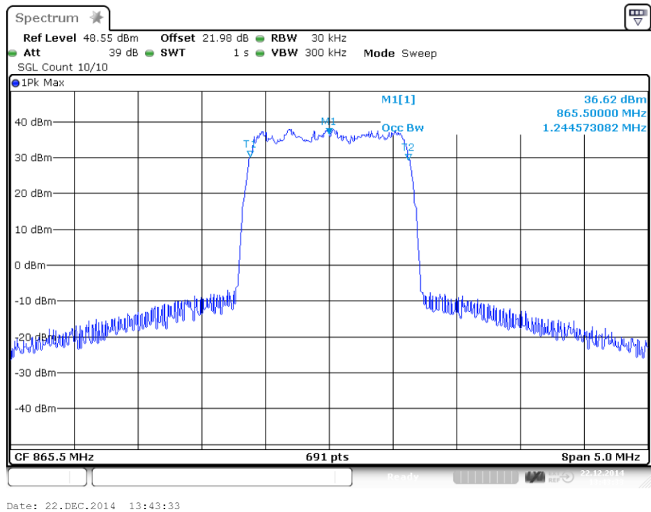
plot 6.3.1.3-#1 Occupied Bandwidth: $90.210, $2.1049; Test results; Downlink; CDMA Output
