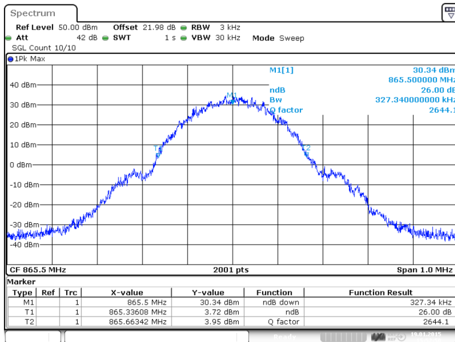
plot 6.3.2.1-#1 Occupied Bandwidth: $90.210, $2.1049; Test results; 26dB BW; GSM Output
