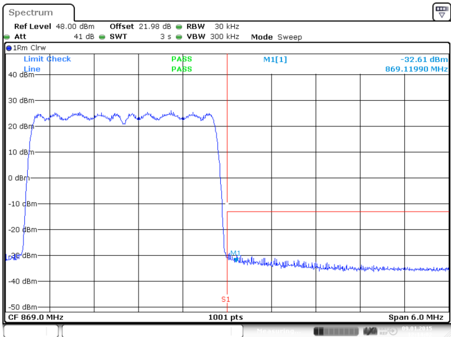
plot 8.3.1.3-#1 Intermodulation: §90.210, §2.1051; Test results; Downlink; CDMA Lower Band Edge
