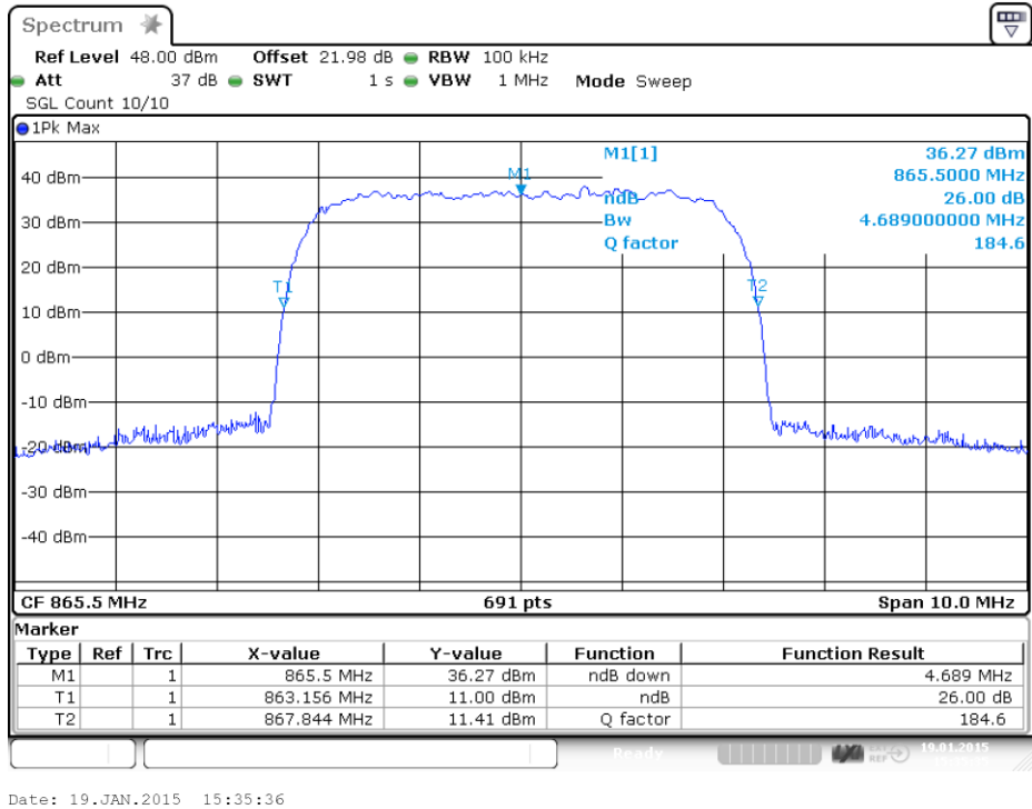
plot 6.3.2.4-#1 Occupied Bandwidth: §90.210, §2.1049; Test results; 26dB BW; WCDMA Output
