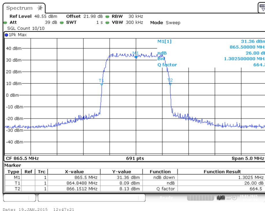
plot 6.3.2.5-#1 Occupied Bandwidth: §90.210, §2.1049; Test results; 26dB BW; LTE Output
