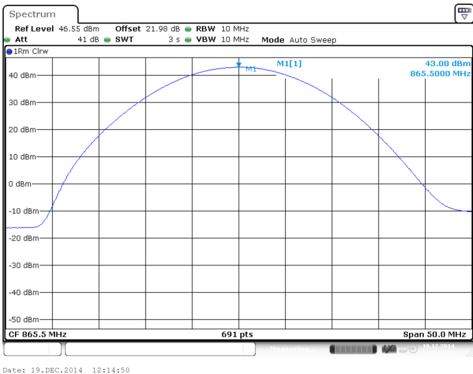
plot 5.3.1.4-#1 RF Power Out: §90.635, §2.1046; Test Results; Downlink; WCDMA Middle
