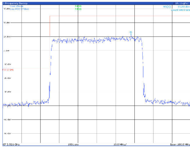
TM3p1, 50 MHz, low channel
