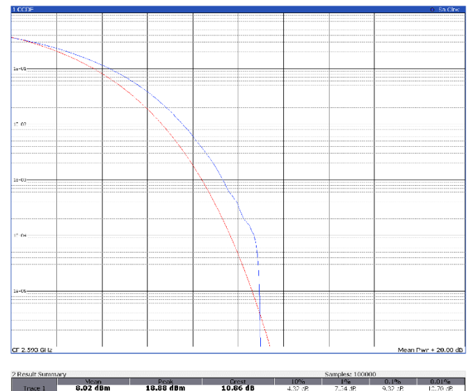
TM3p1a, 100 MHz, mid channel
