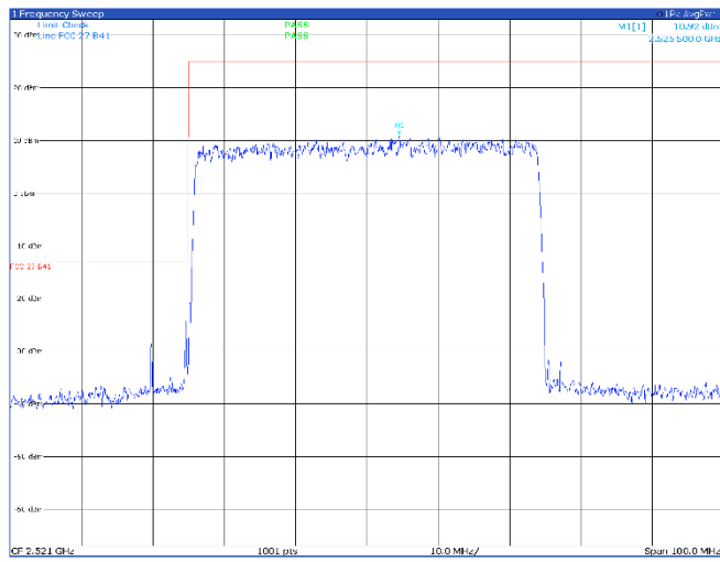
TM3p3, 50 MHz, low channel
