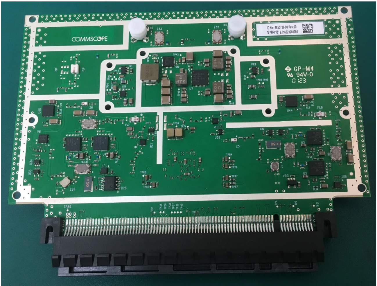
RM 34T – Assembled PCB 7855726-00- Internal picture
