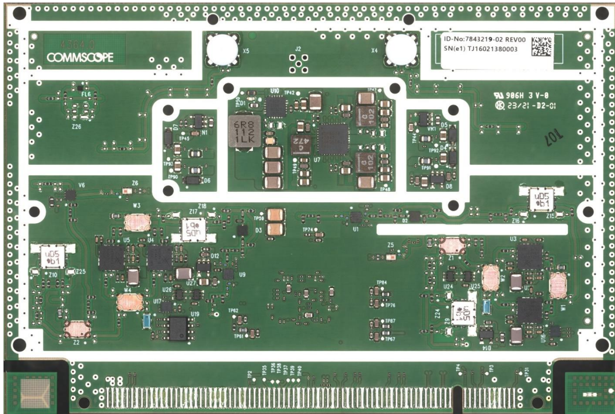
TOP View
