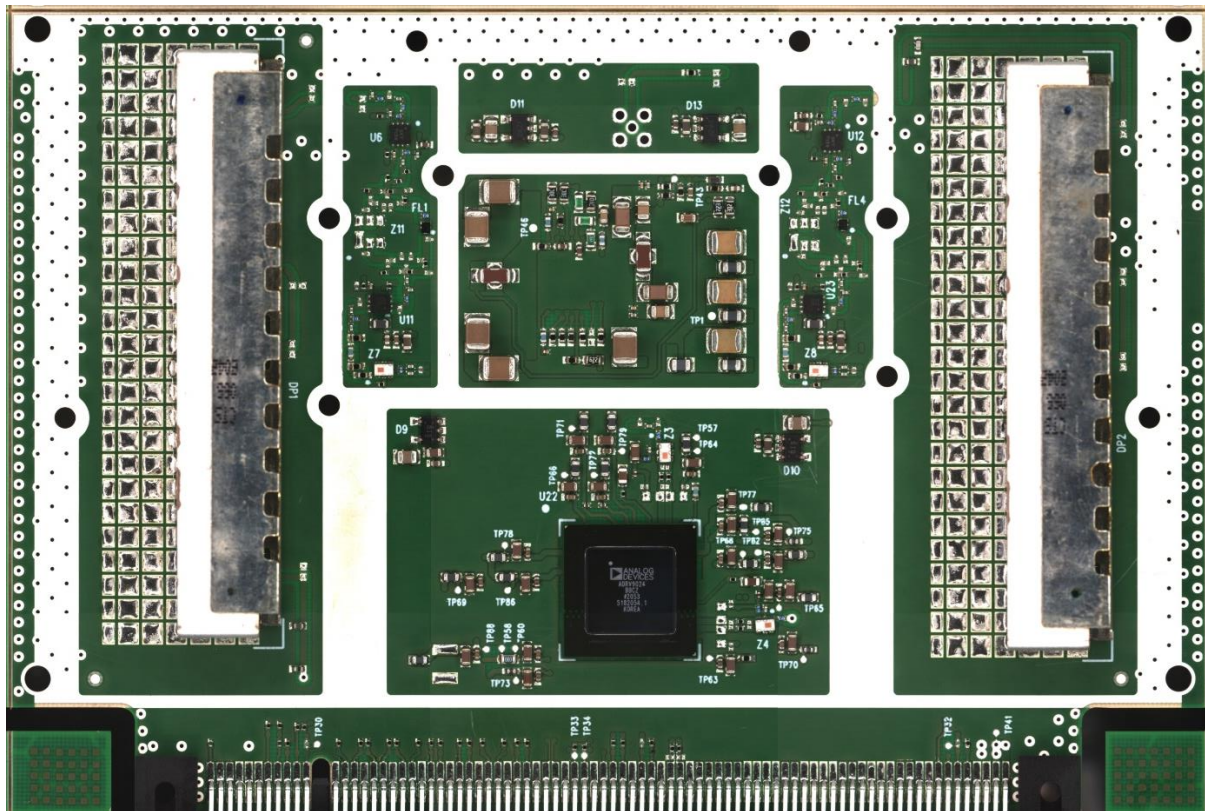
BOTTOM View
