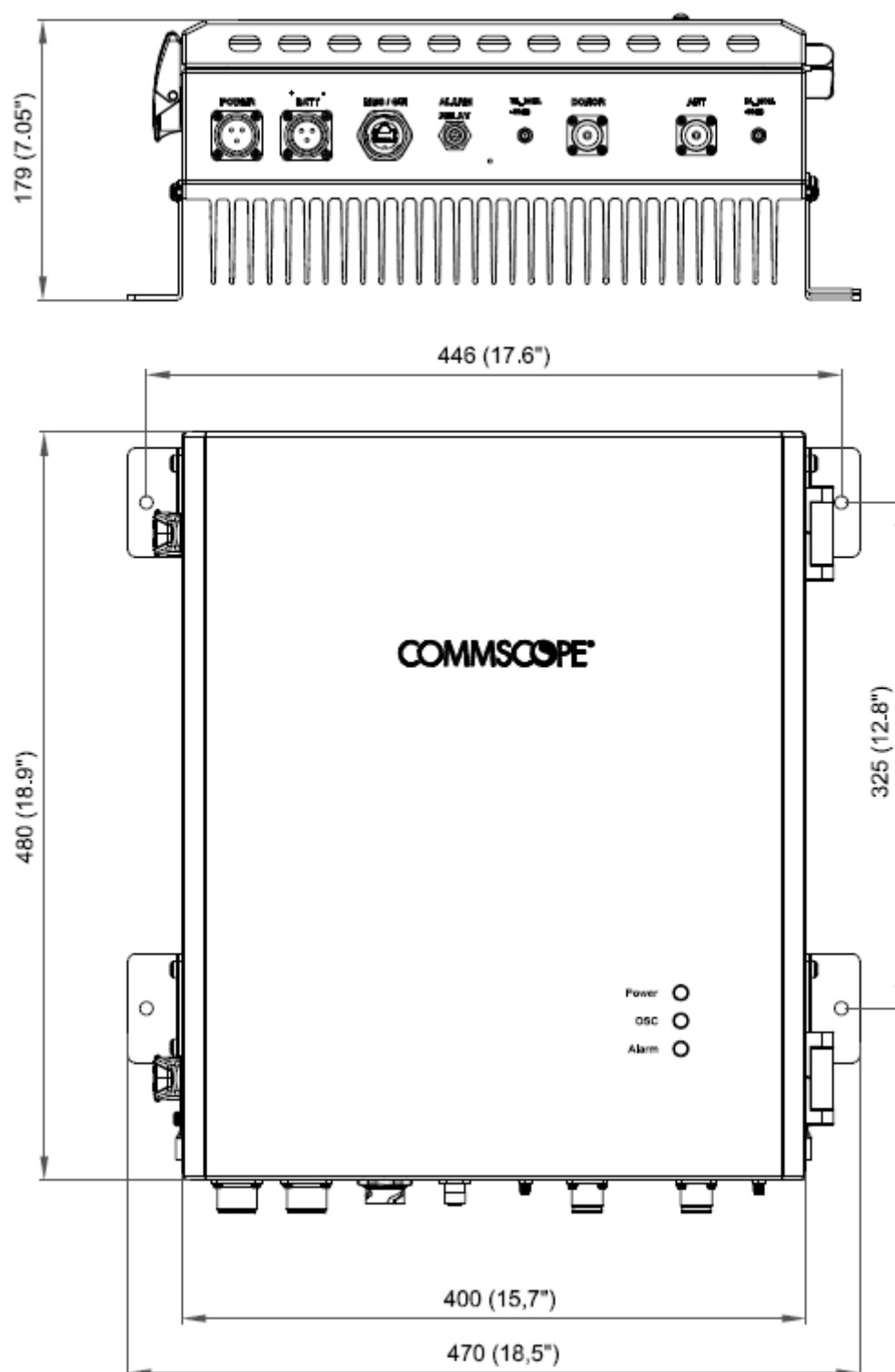
figure 8-2 Cabinet measurements
