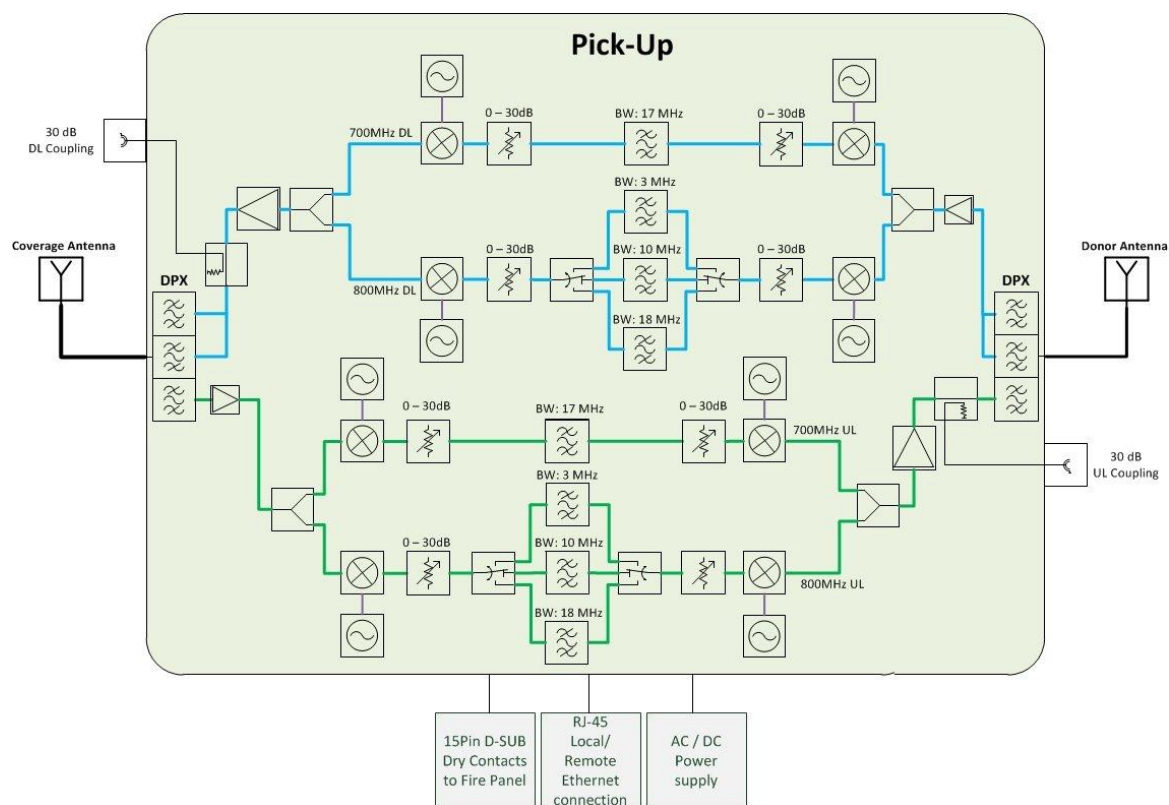
figure 3-1 Configuration of a PSR 700/800 MHz 0.5/2W, analogue variant
