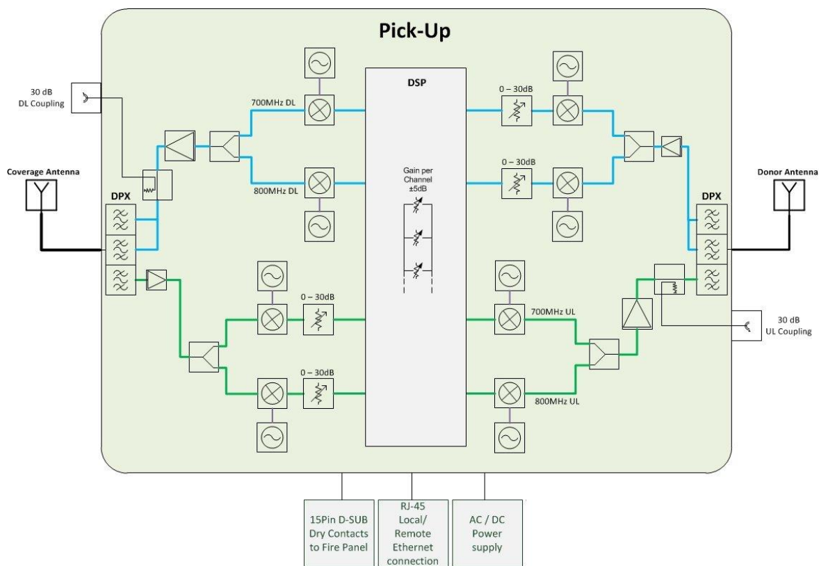
figure 3-2 Configuration of a PSR 700/800 MHz 0.5/2W, digital variant
