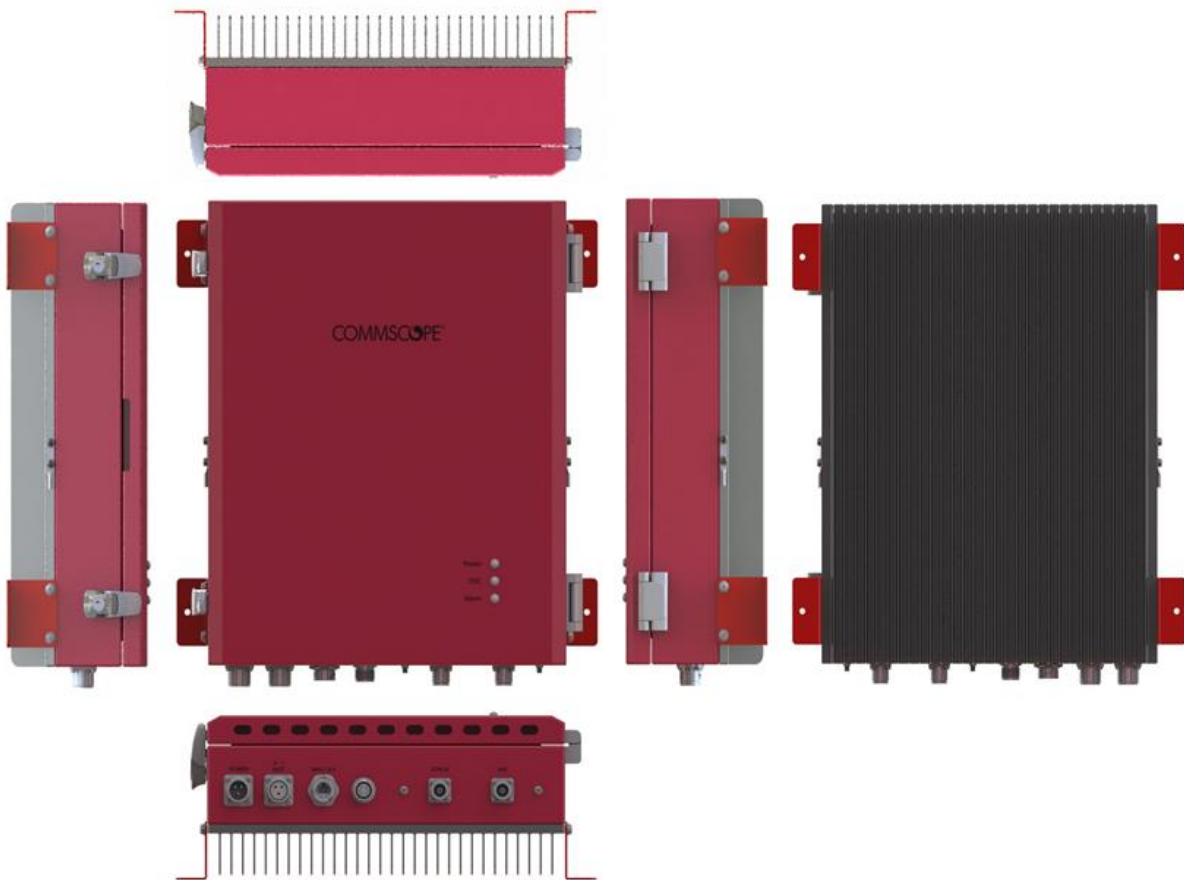
figure 8-1 External configuration
