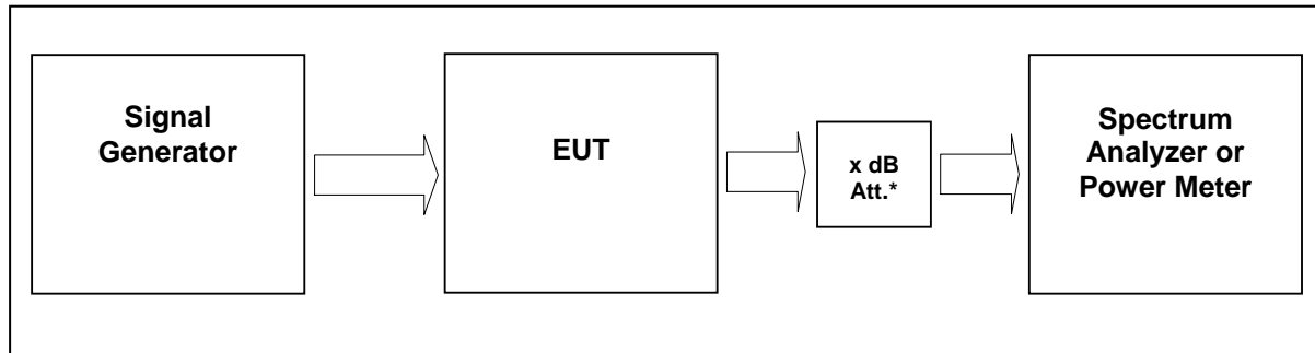
External Attenuator DL x dB = 30 dB figure 5-#1 Test setup: RF Power Out: §27.50, §2.1046; RSS-131, RSS-GEN
