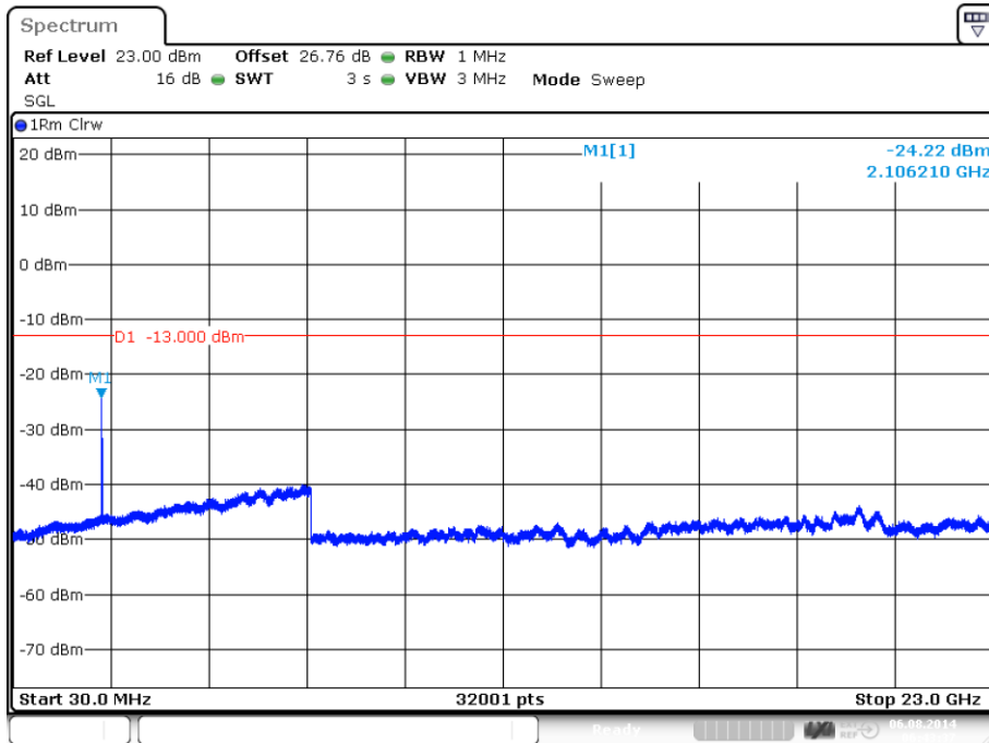
plot 7.3.1.4-#1 Spurious Emissions at Antenna Terminals: §27.53, §2.1051; Test results; Downlink; CDMA > 1MHz to band edge; carrier (2132,5MHz) notched
