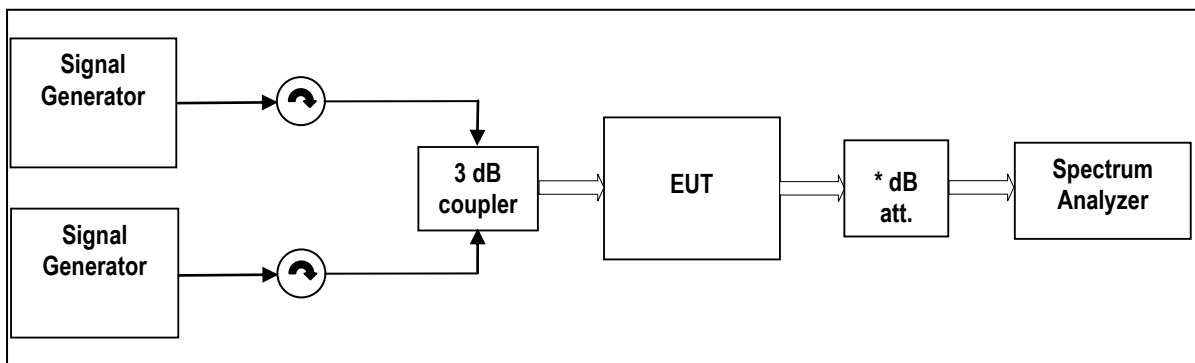
External Attenuator DL x dB = 20 dB
