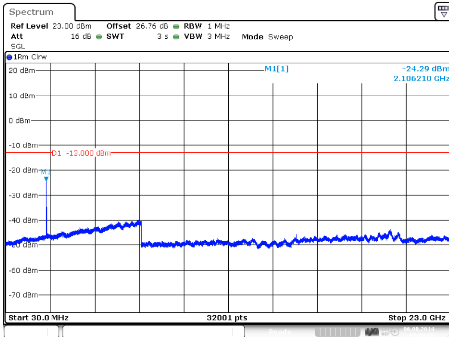
plot 7.3.1.5-#1 Spurious Emissions at Antenna Terminals: §27.53, §2.1051; Test results; Downlink; W-CDMA > 1MHz to band edge; carrier (2132,5MHz) notched
