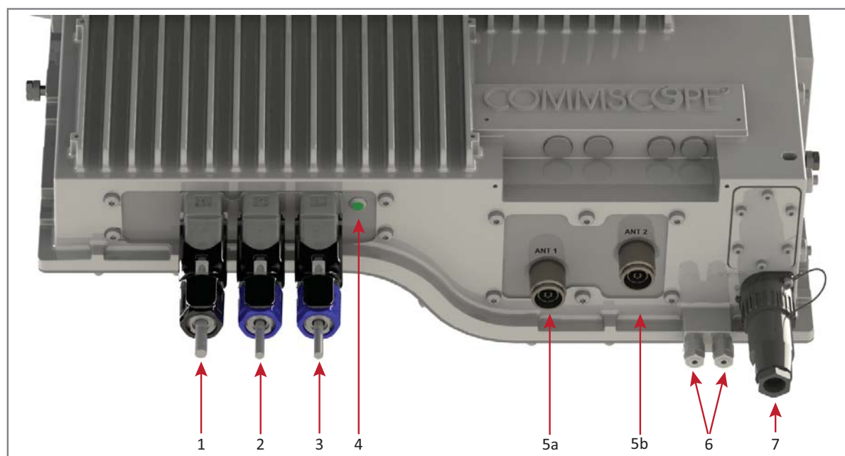
Figure 3. Location of Connectors and Power LED on a CAP M with Two Antenna Connectors
