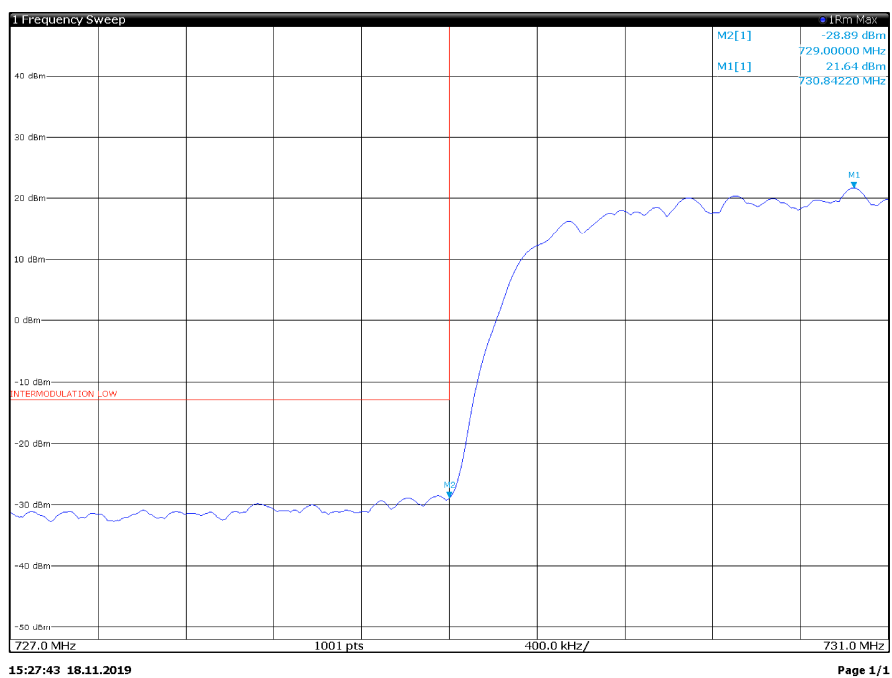
Lower block edge intermodulation products with input at AGC threshold, Antenna 2
