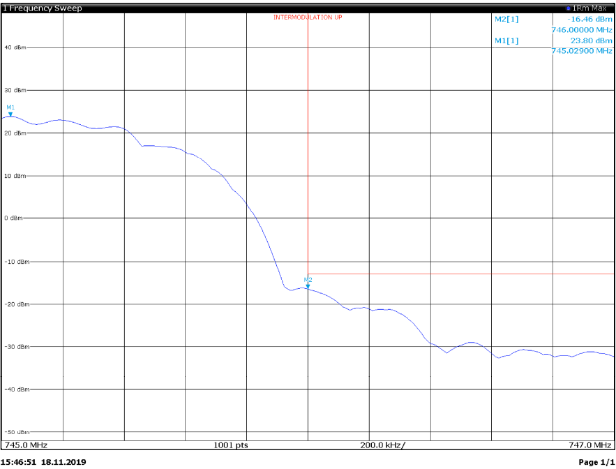
Upper block edge with input at AGC threshold + 3 dB, Antenna 2
