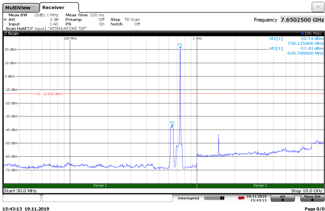
Spurious conducted emissions with input at AGC threshold at 737.5 MHz, Antenna 2
