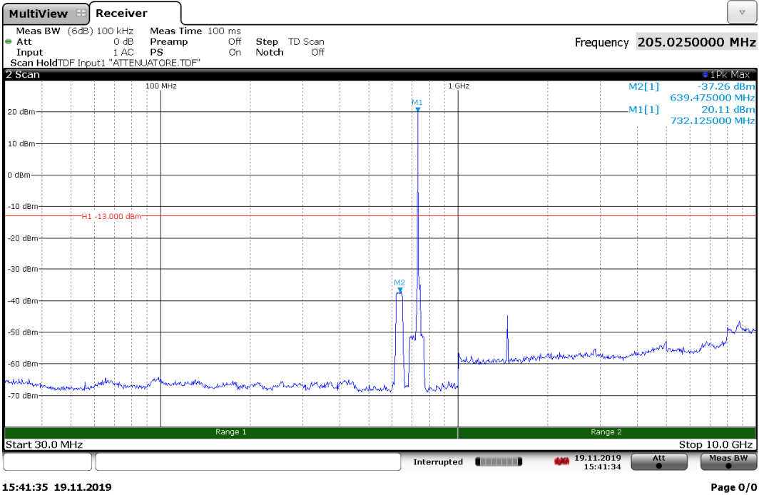
Spurious conducted emissions with input at AGC threshold at 731.5 MHz, Antenna 2
