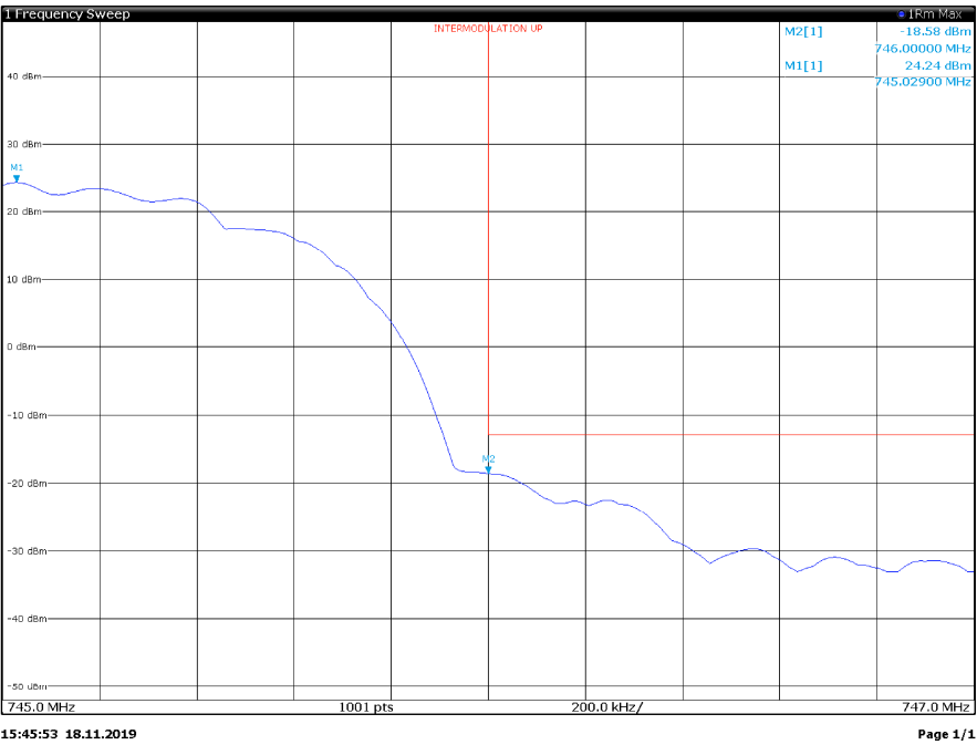
Upper block edge with input at AGC threshold, Antenna 2
