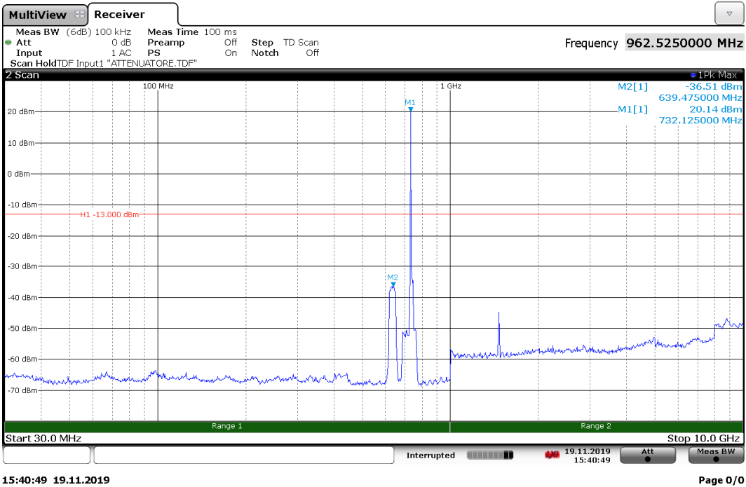
Spurious conducted emissions with input at AGC threshold at 731.5 MHz, Antenna 1
