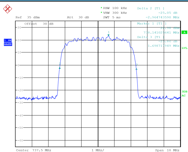
Output Antenna 1
