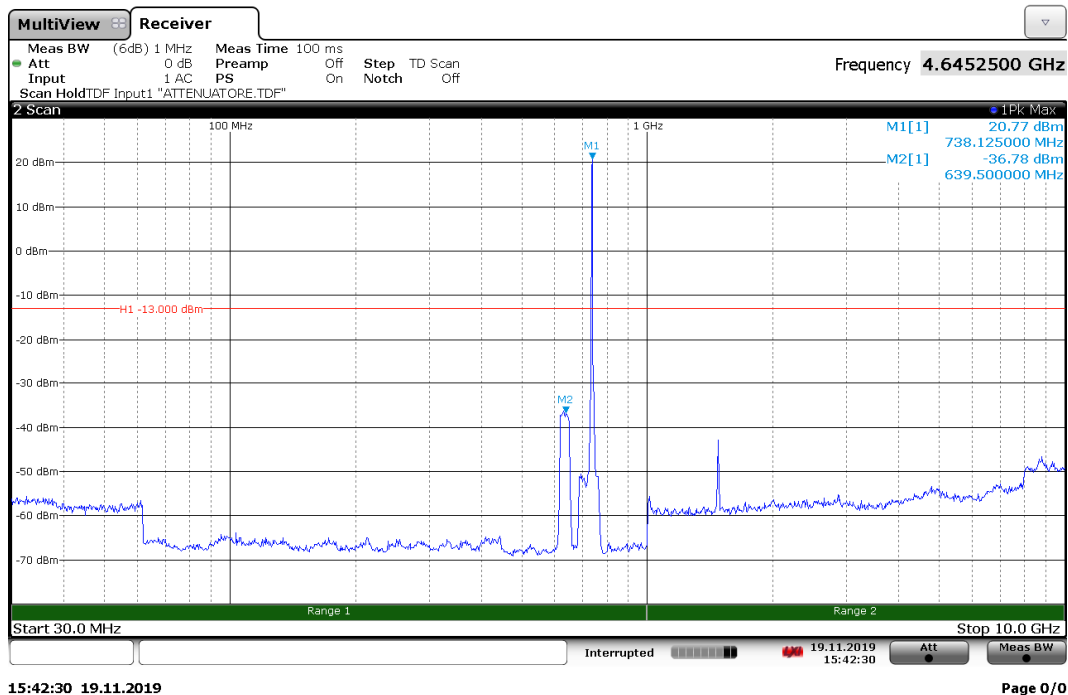
Spurious conducted emissions with input at AGC threshold at 737.5 MHz, Antenna 1
