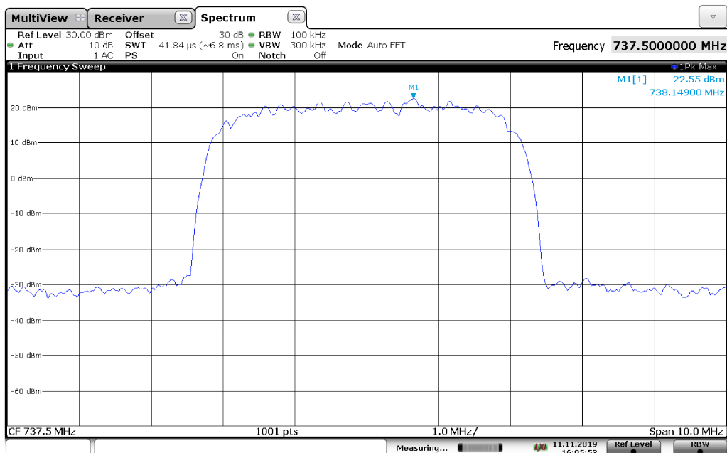
Output spectral plot with input at AGC threshold with AWGN5 signal at 737.5 MHz, Antenna 2
