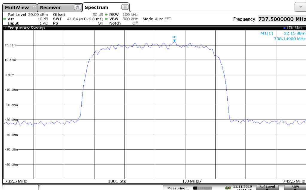
Output spectral plot with input at AGC threshold + 1 dB with AWGN5 signal at 737.5 MHz, Antenna 1
