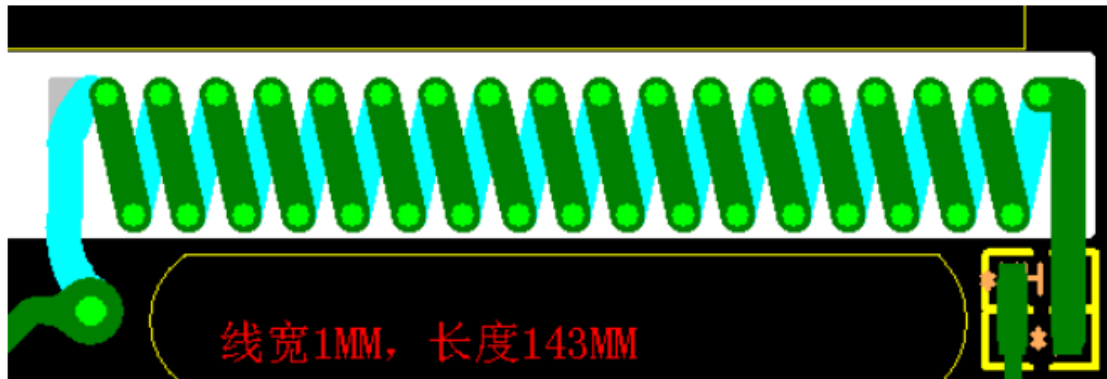
Antenna diagram
