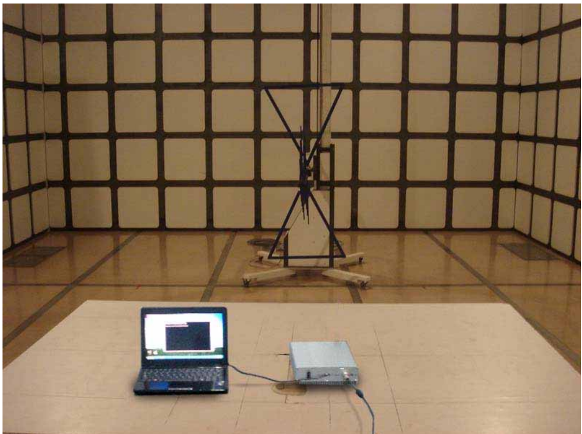
Radiated Emission
