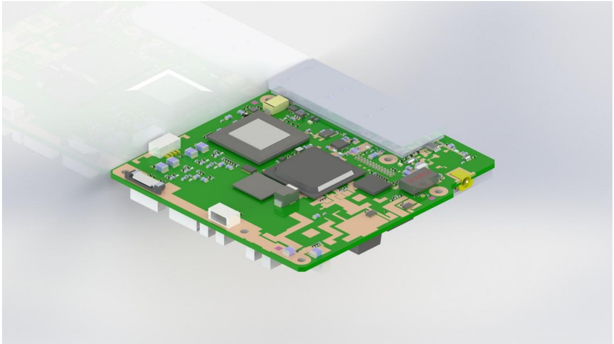
Underside Render (solid works)
