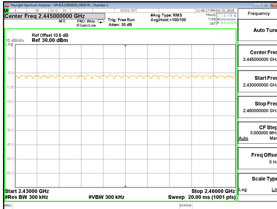
NUMBER OF HOPPING CHANNELS (30 MHz SPAN, SECOND SEGMENT)
