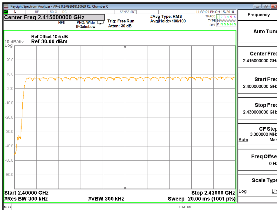
NUMBER OF HOPPING CHANNELS (30 MHz SPAN, FIRST SEGMENT)
