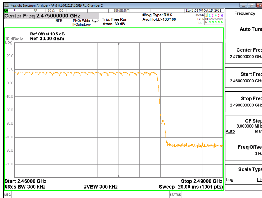
NUMBER OF HOPPING CHANNELS (30 MHz SPAN, THIRD SEGMENT)
