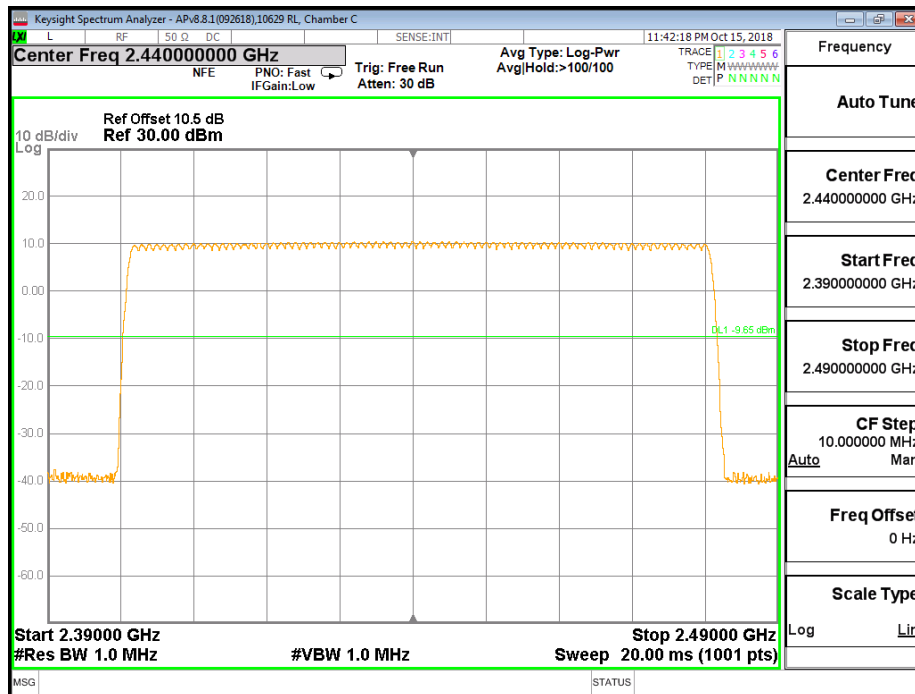
NUMBER OF HOPPING CHANNELS (100 MHz SPAN)
