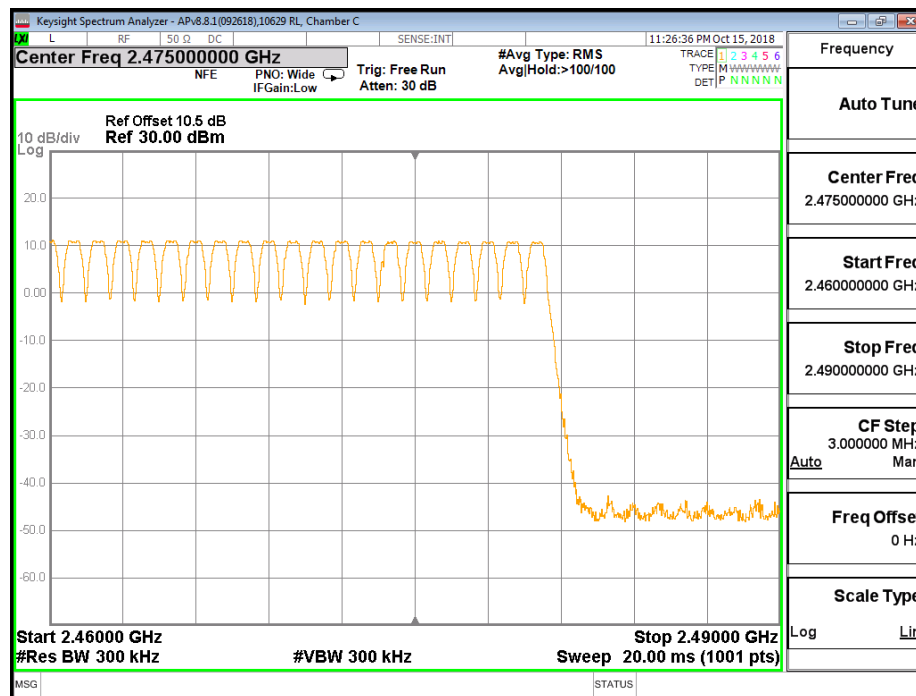
NUMBER OF HOPPING CHANNELS (30 MHz SPAN, THIRD SEGMENT)
