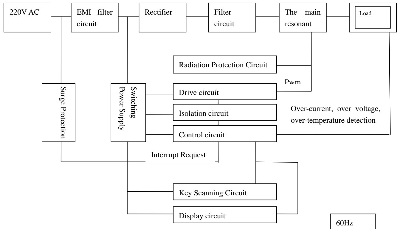
BS20-SC1 block diagram
