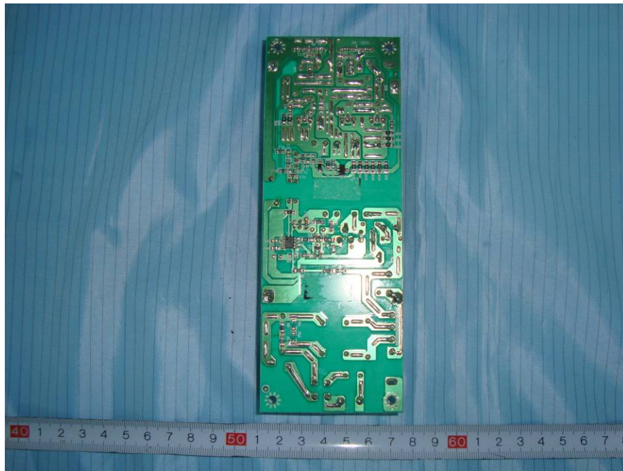
EUT – Power Supply Board Circuit View
