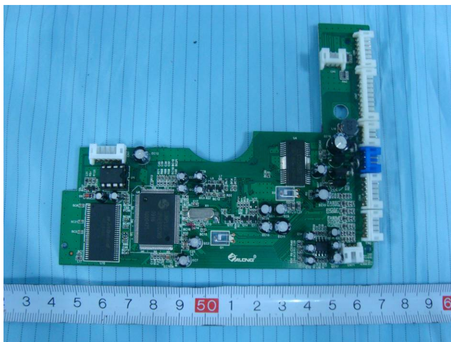
EUT – DVD Control Board Components View
