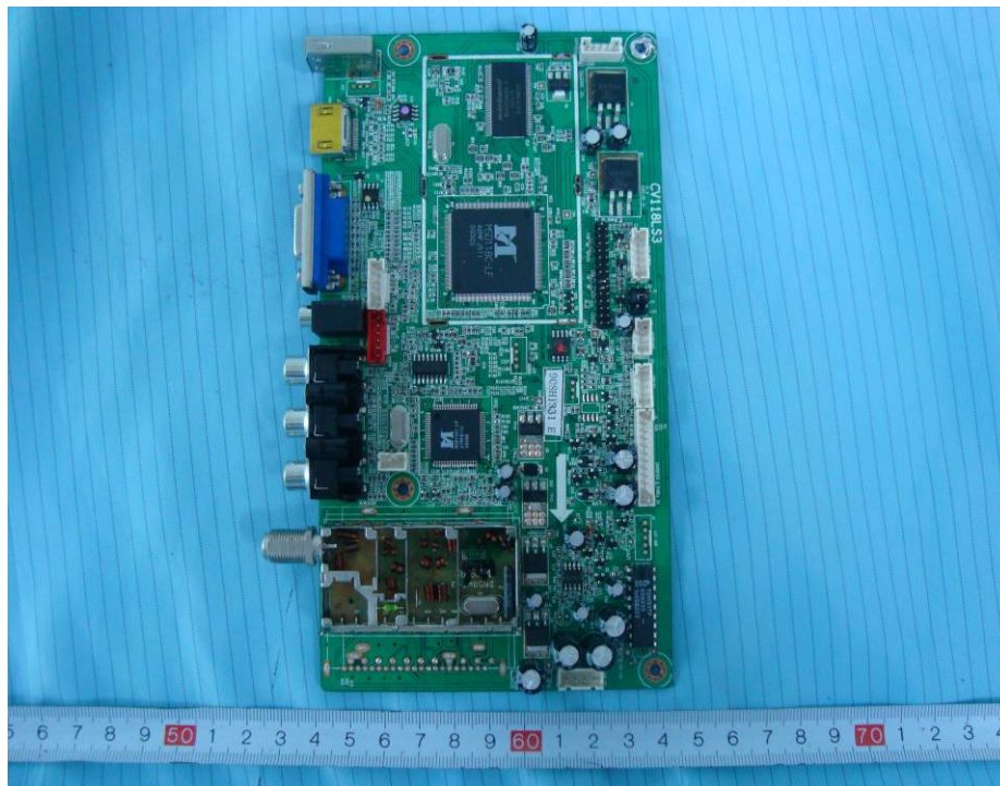
EUT – Main Board Components View
