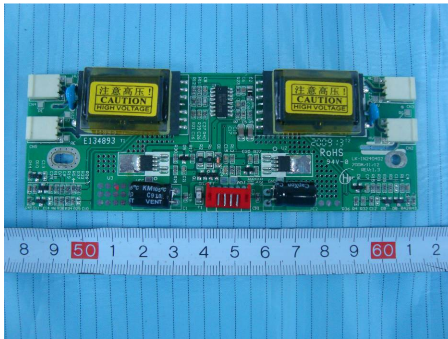
EUT – Converter Components View
