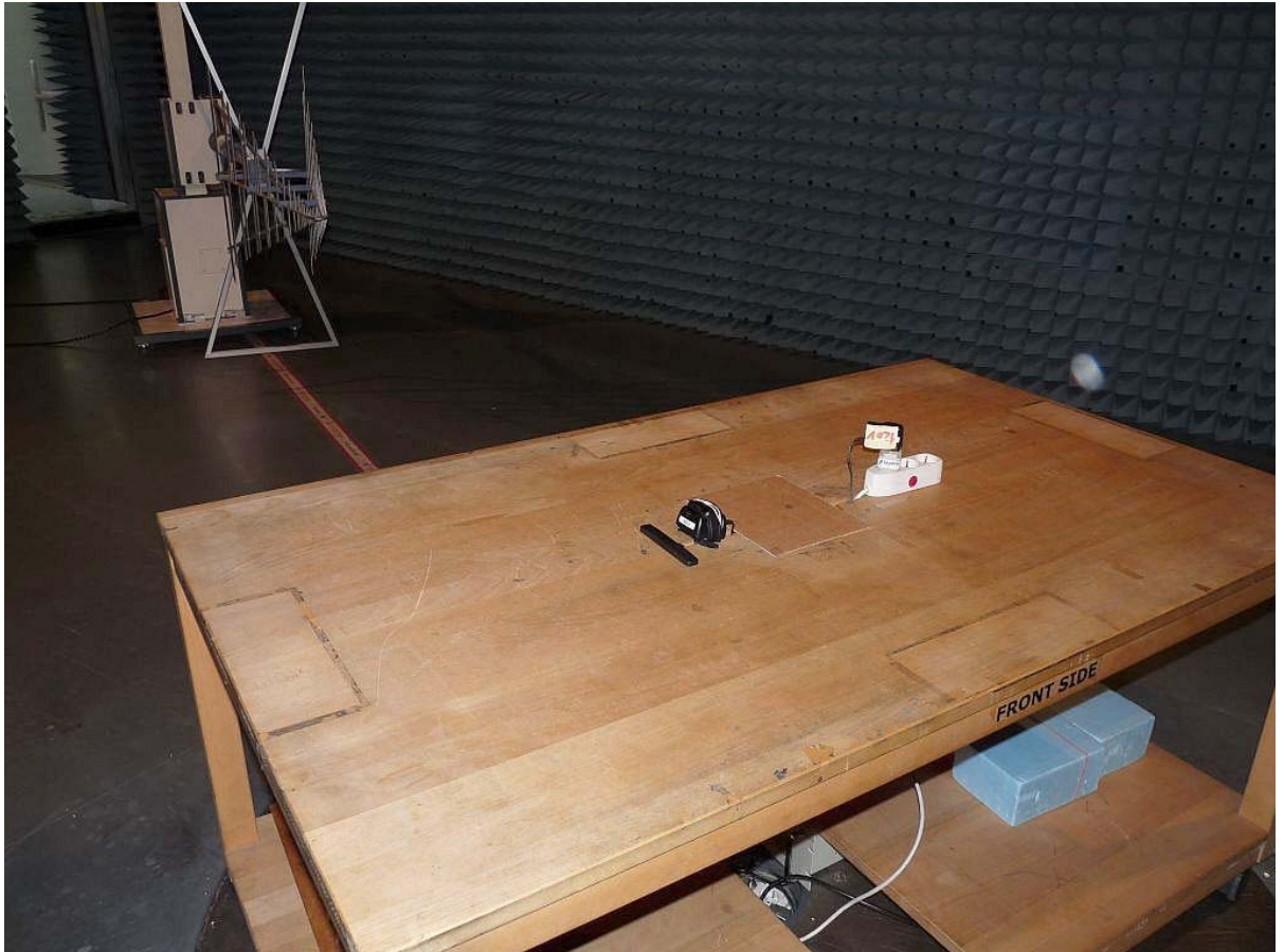
Test setup for the test radiated emissions
