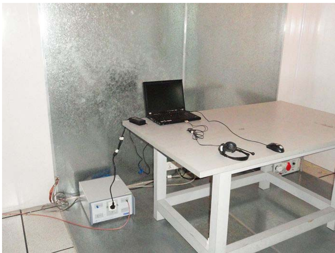
Conducted Emission test view
