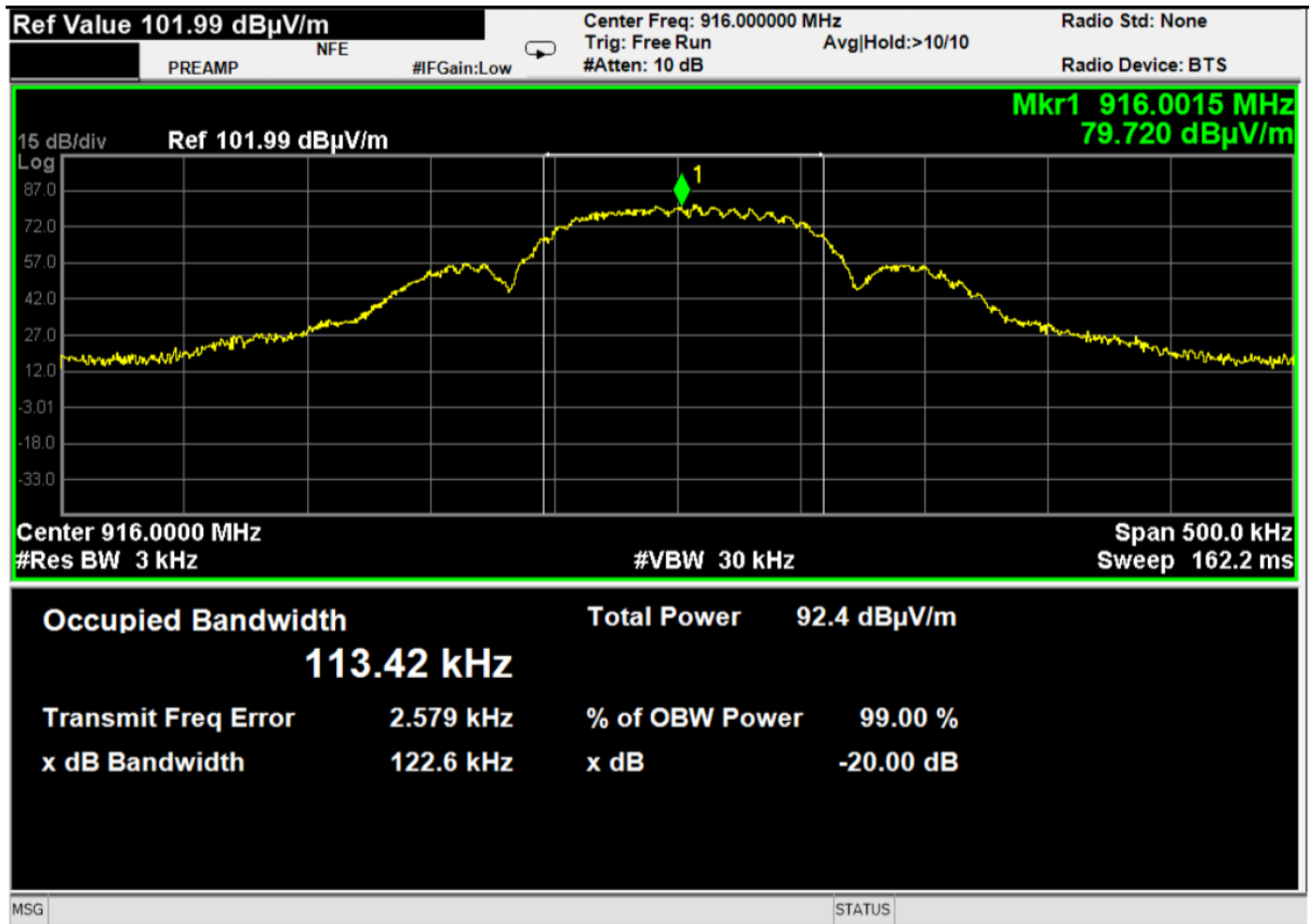
99 Percent Bandwidth Plot – 916.00 MHz
