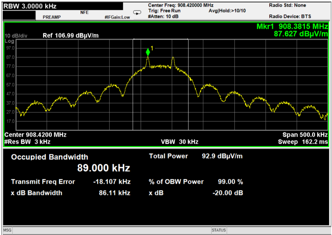
99 Percent Bandwidth Plot – 908.42 MHz
