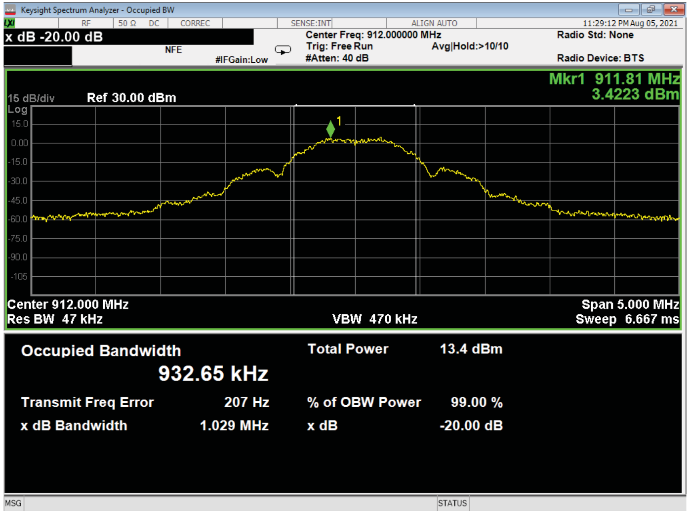
99% Bandwidth Plot – 912 MHz
