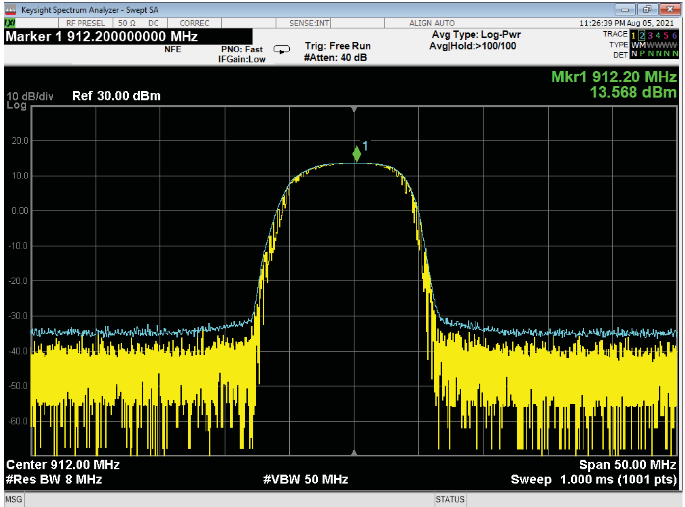
Peak Power Output – Low Channel
