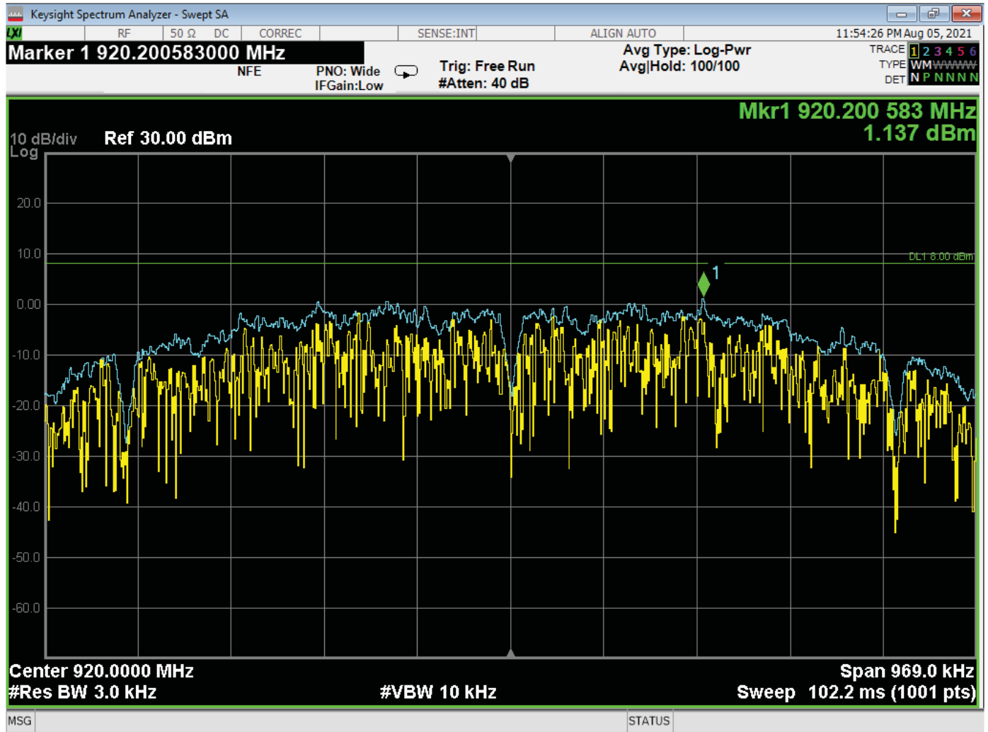
Peak Power Spectral Density – High Channel
