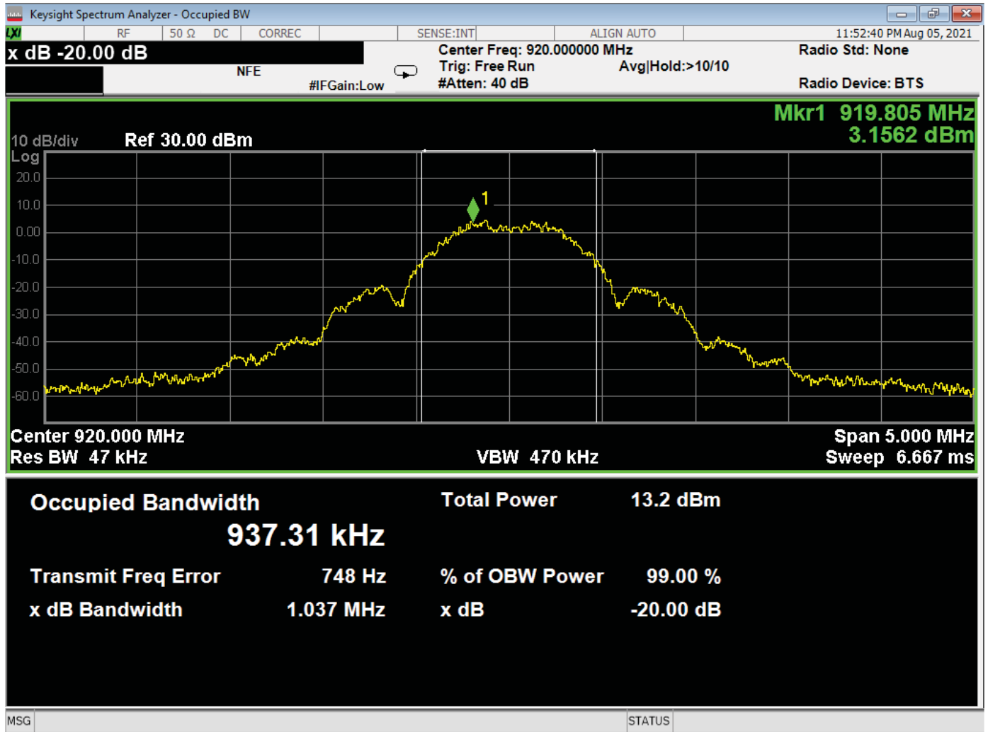
99% Bandwidth Plot – 920 MHz
