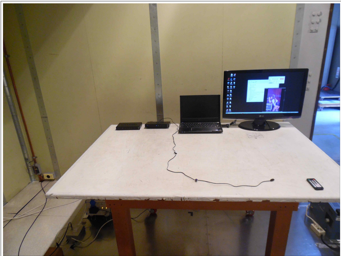
Conducted Disturbance Voltage (Communication)
