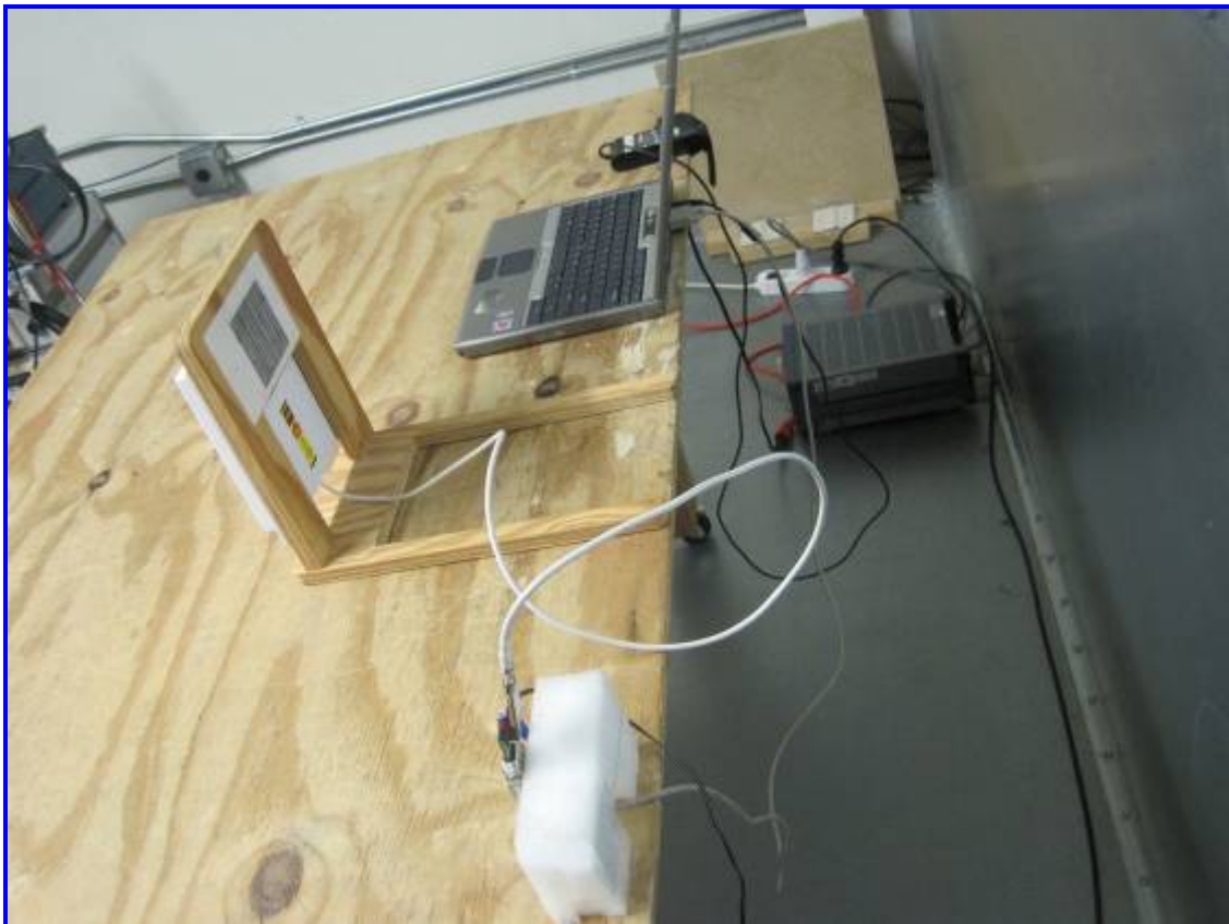
Conducted Emission Test Setup (Flat Patch Antenna) – Rear View
