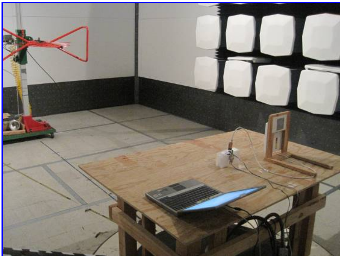
Radiated Emission Test Setup (Flat Patch Antenna) – Rear View
