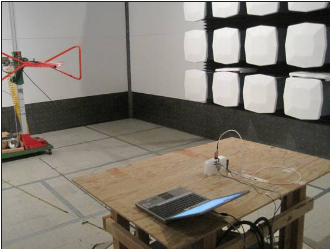
Radiated Emission Test Setup (Near Field Antenna) – Rear View
