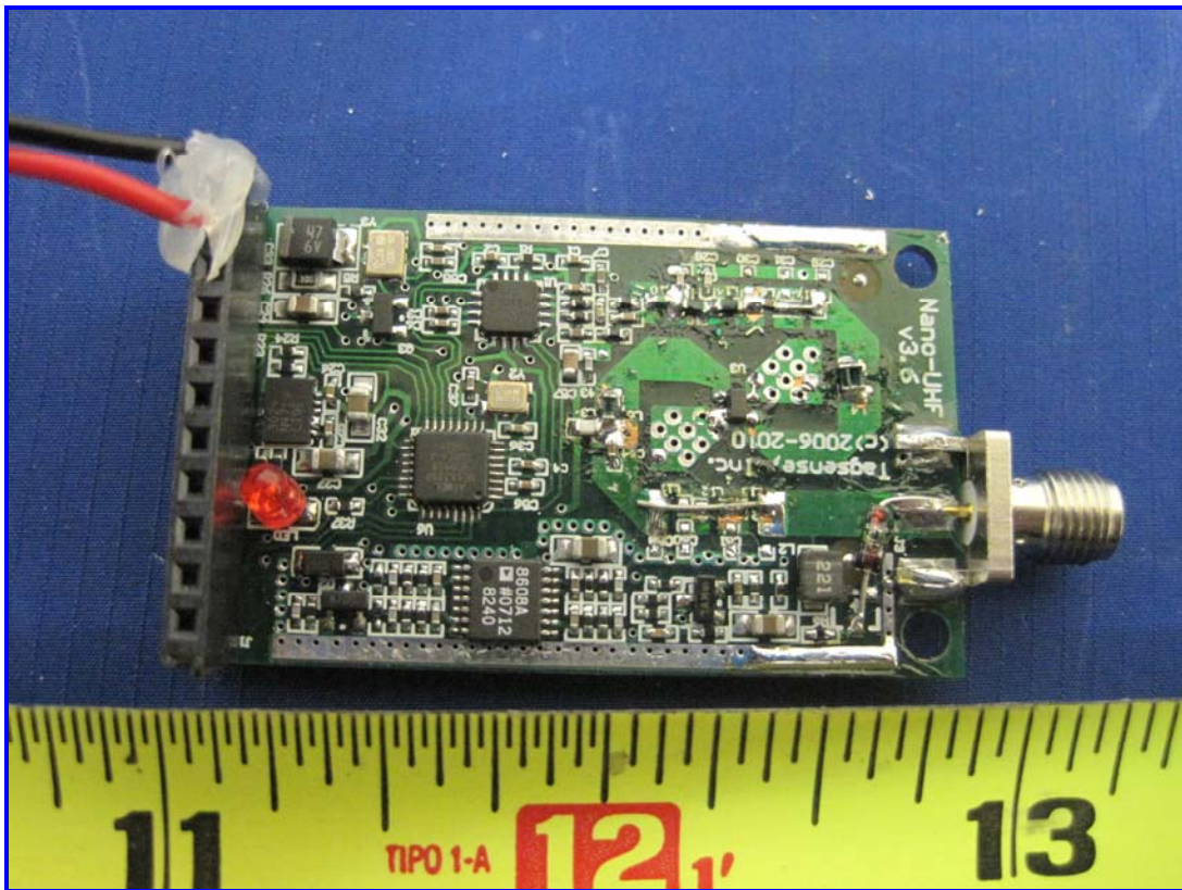
Component View without RF Shield
