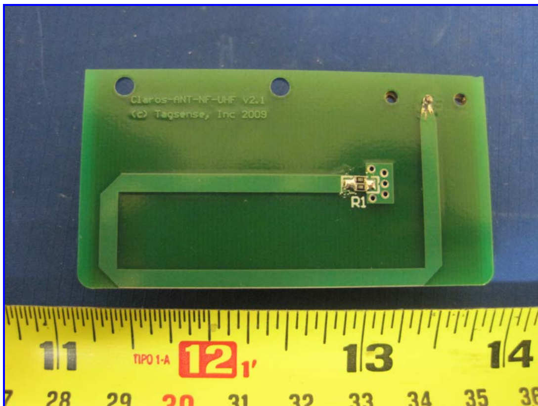
Near Field Antenna – Antenna PCBA Solder View
