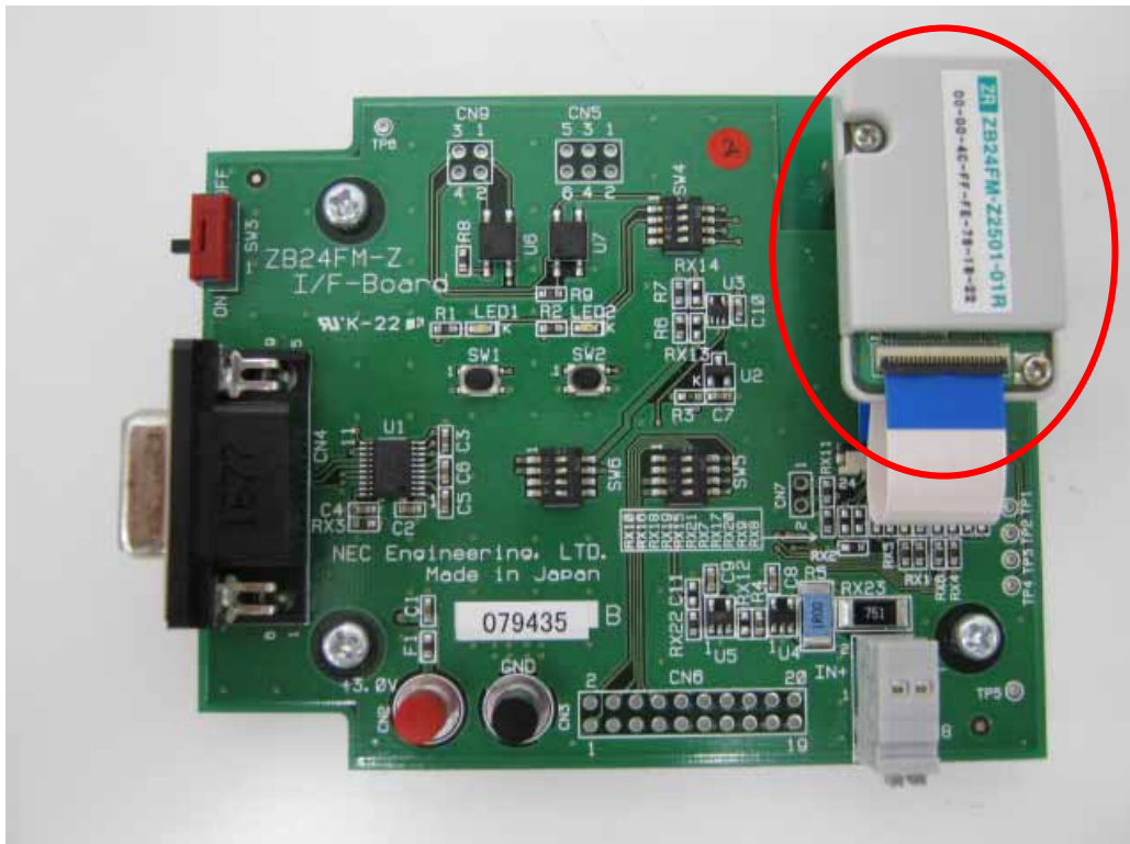
PCB for testing (Transmitter WDT)
