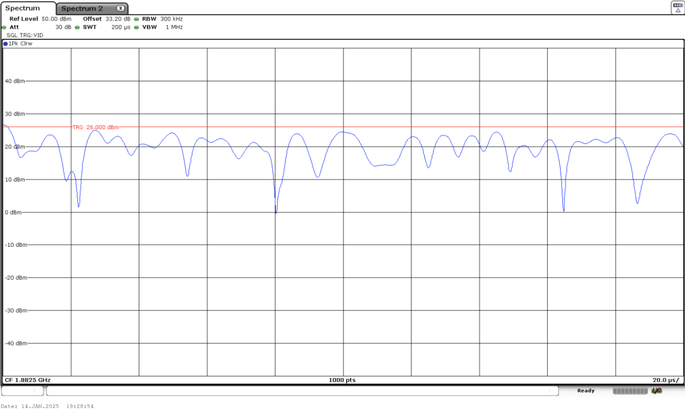
LTE Cat 1bis Band 2: BW=1.4 MHz. 16QAM. RB Size=1. RB Offset=0. Middle Channel.
