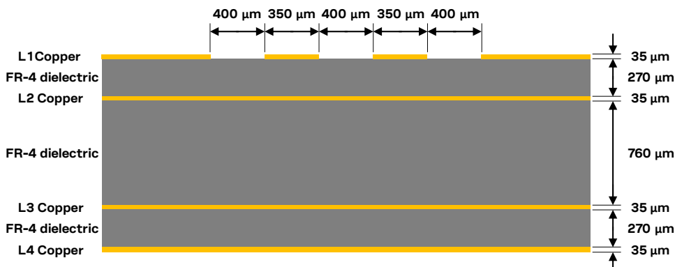
Figure 53: Example of USB line design, with Z_0 close to 90 \Omega and Z_{CM} close to 30 \Omega , for the described 4-layer board layup
