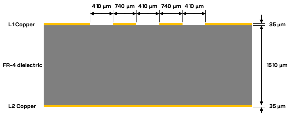
Figure 54: Example of USB line design, with Z_0 close to 90 \Omega and Z_{CM} close to 30 \Omega , for the described 2-layer board layup
