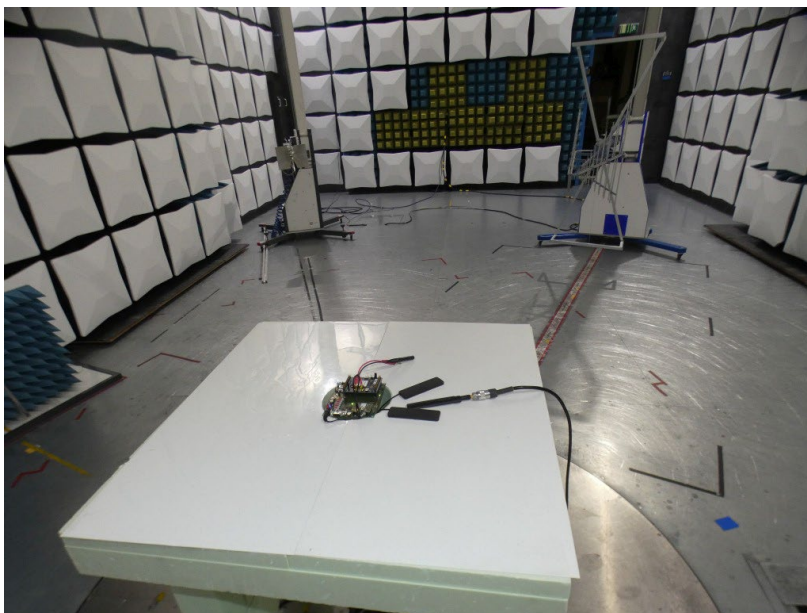
Photo 6: Test Antenna
