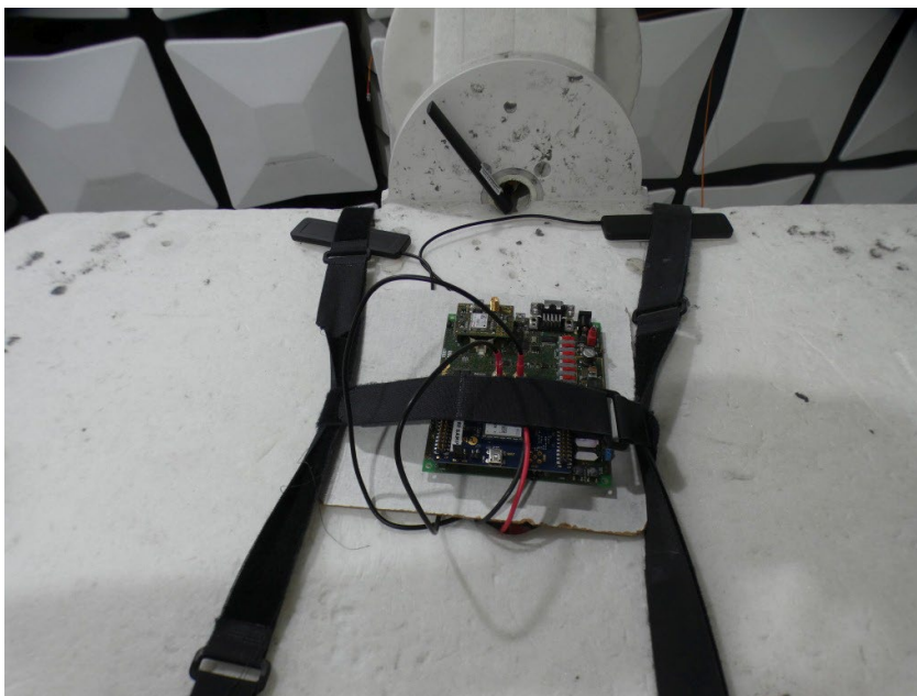
Photo 2: EUT setup
