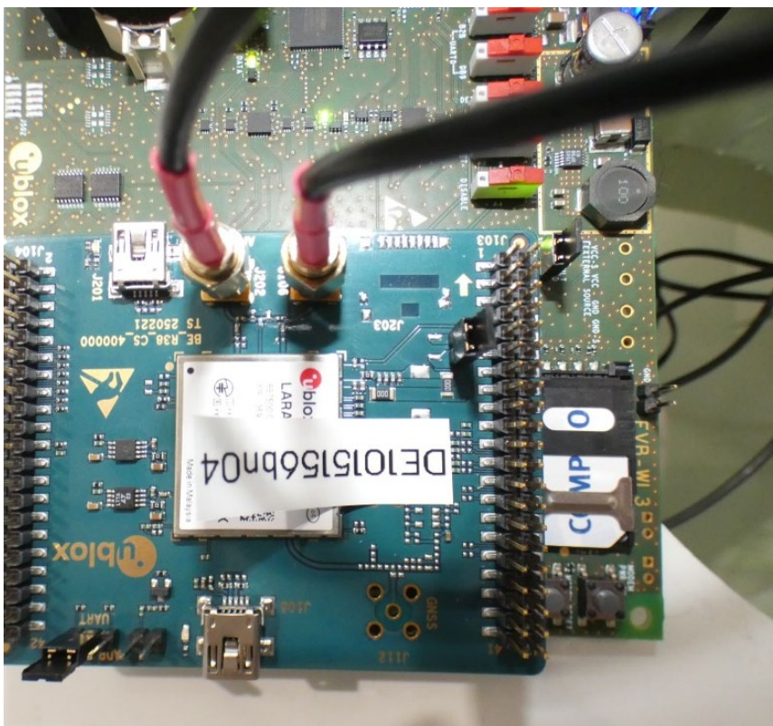
Photo 5: EUT (top side)
