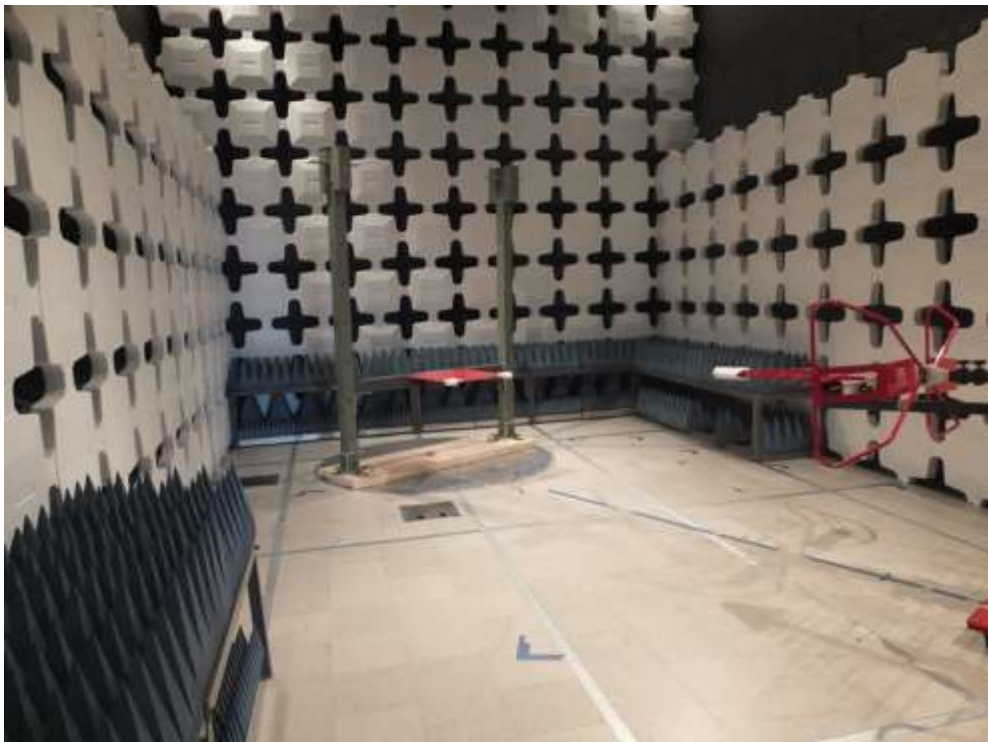
Test Facility (Setup for Radiated Emission 30MHz – 1000MHz)
