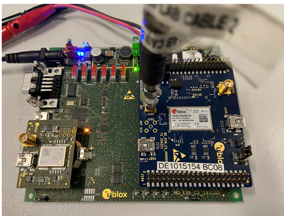
Photo 3: EUT (top side) SARA-R422M10S End of report
