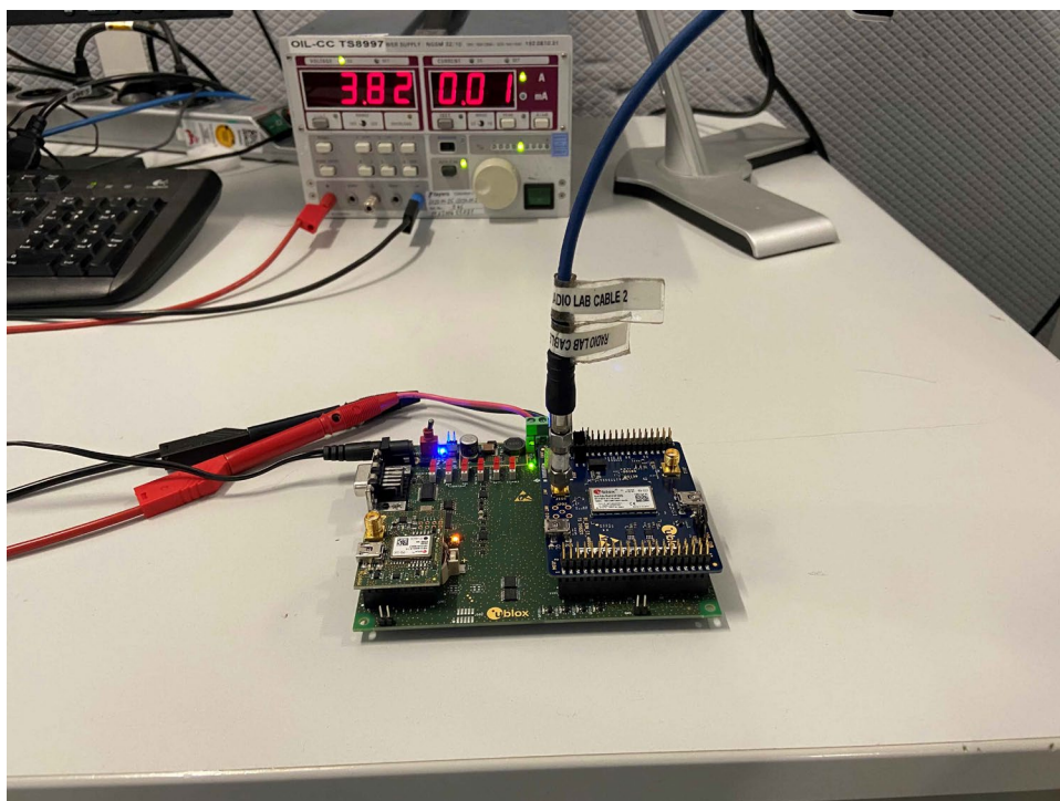
Photo 2: EUT setup for conducted measurements SARA-R422M10S
