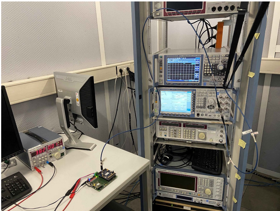
Photo 1: Test setup for conducted measurements SARA-R422M10S
