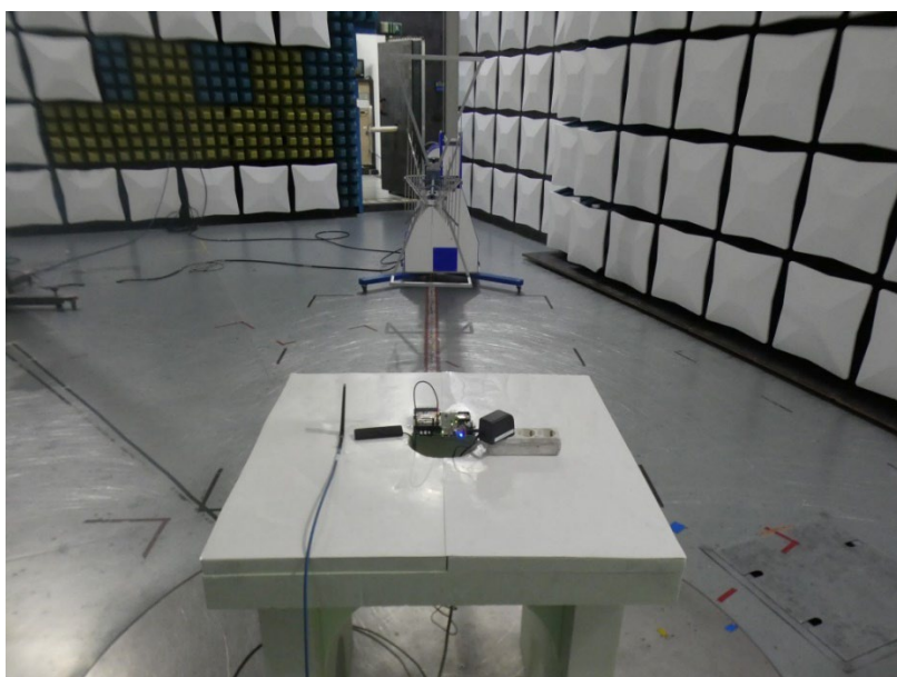
Photo 2: Test setup for radiated measurements (below 1GHz)
