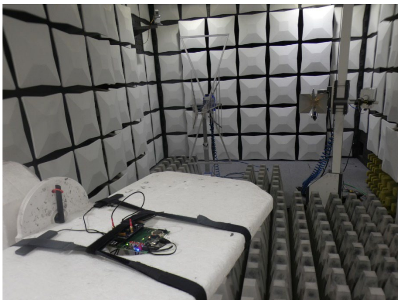
Photo 1: Test setup for radiated measurements
