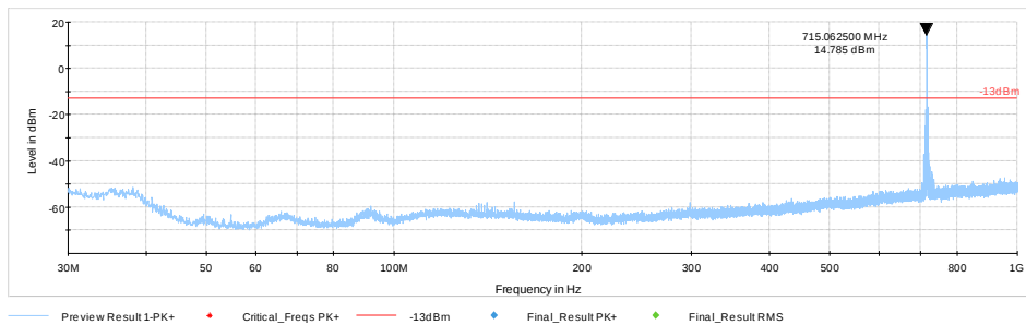
Plot #30 Radiated Emissions: 30 MHz – 1GHz
