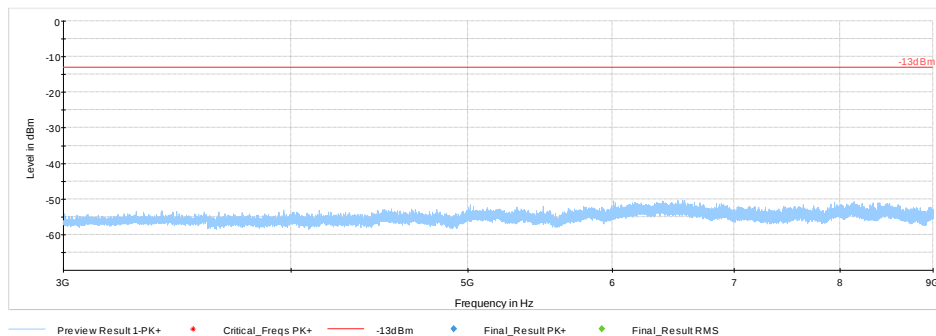
Plot #39 Radiated Emissions: 3-9 GHz
