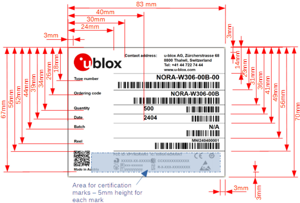
Figure 2: NORA-W3xx batch label, dimensioned drawing
