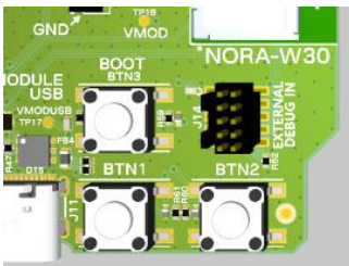
Figure 8: BOOT (BTN3) button to enter the bootloader
