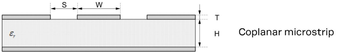
Figure 21: Coplanar micro-strip dimensions
