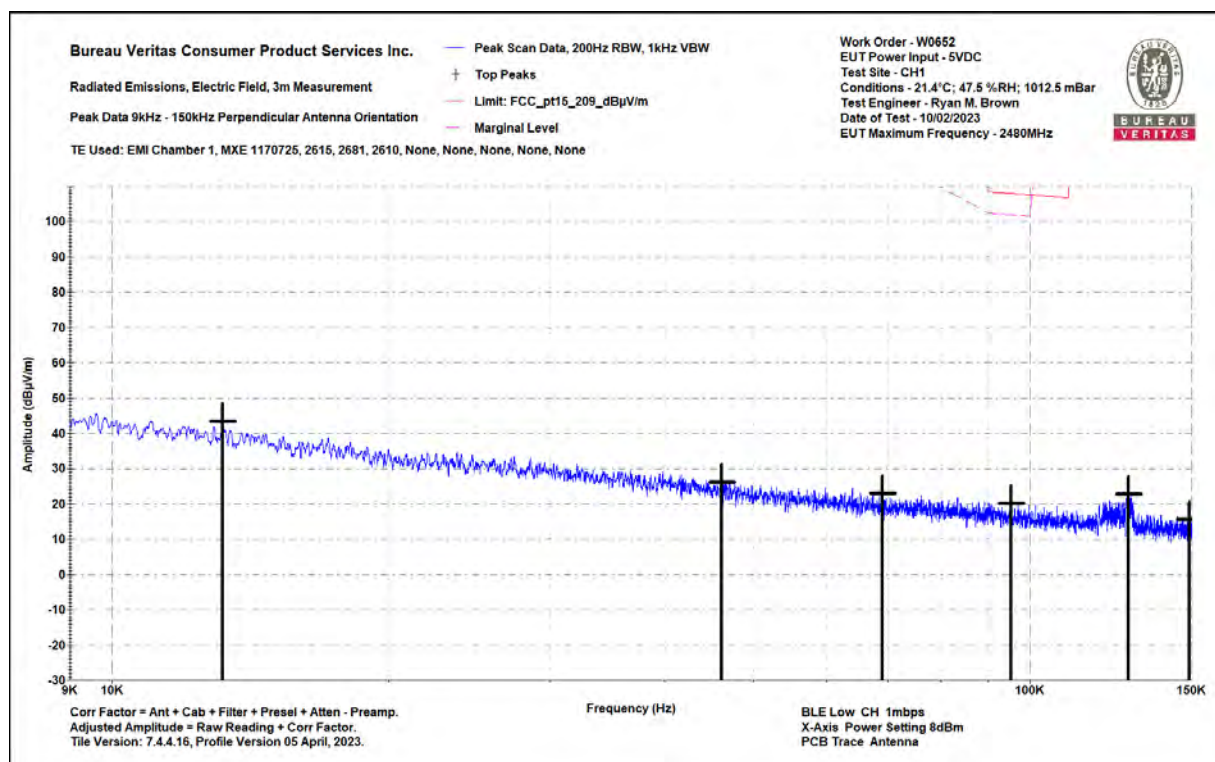
0.009-0.15MHz Perpendicular
