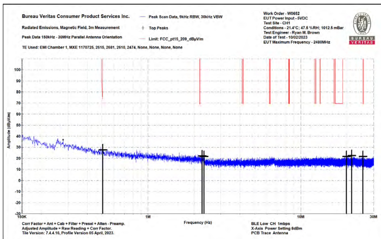
0.15-30MHz Parallel
