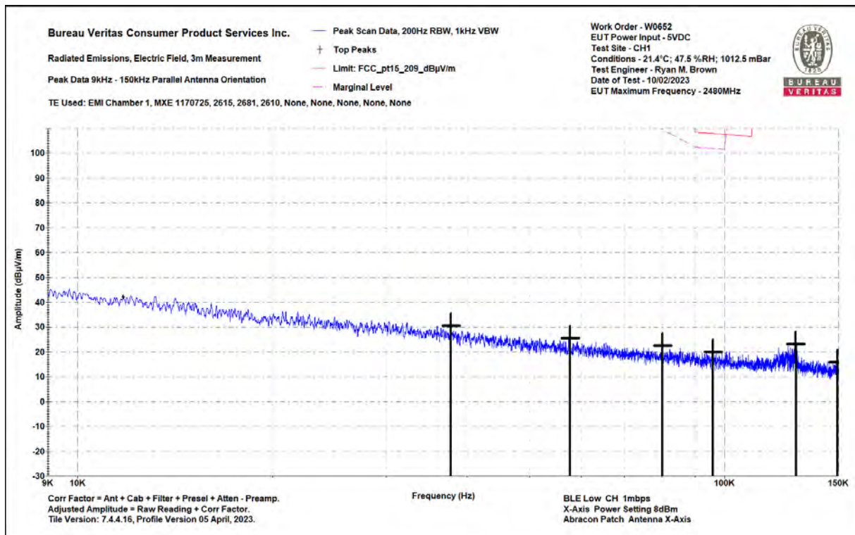
0.009-0.15MHz Parallel
