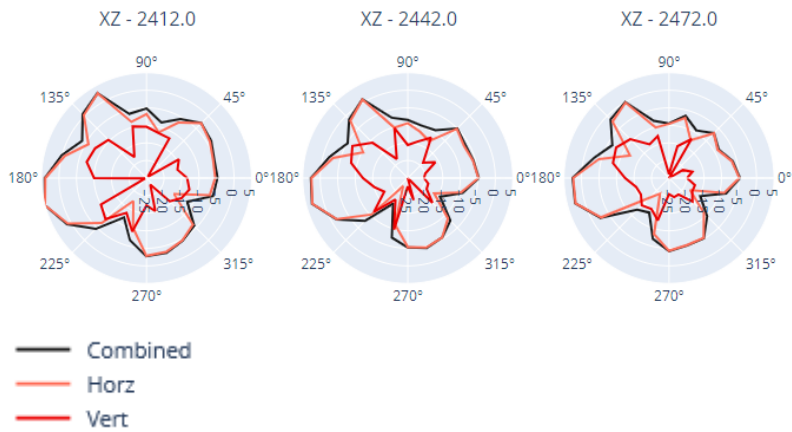
Figure 6: ANT-X100P001B24553 antenna – 2.4 GHz, 2D X-Z plane radiation pattern
