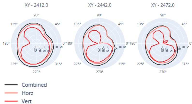
Figure 4: ANT X100P001B24553 antenna – 2.4 GHz, 2D X-Y plane radiation pattern
