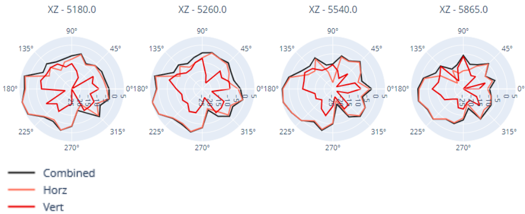
Figure 7: ANT-X100P001B24553 antenna – 5 GHz, 2D X-Z plane radiation pattern
