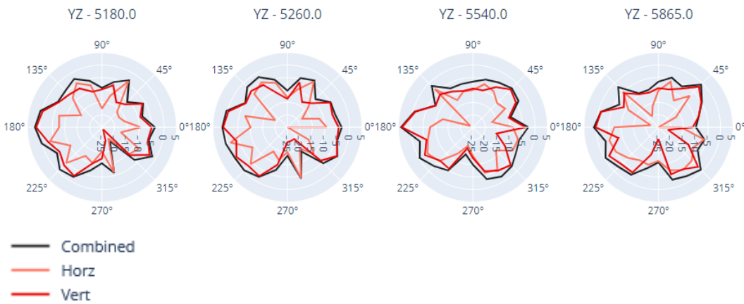
Figure 9: ANT-X100P001B24553 antenna – 5 GHz, 2D Y-Z plane radiation pattern
