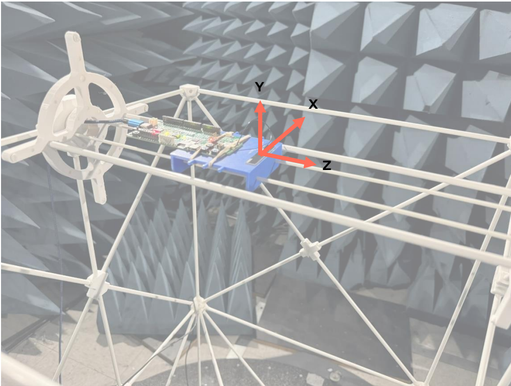
Figure 2: ANT-X100P001B24553 connected to NORA-W3, mounted in chamber
