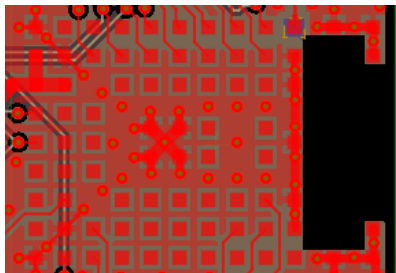
Figure 24: NORA-W3x6 keepout – not required for NORA-W3x1
