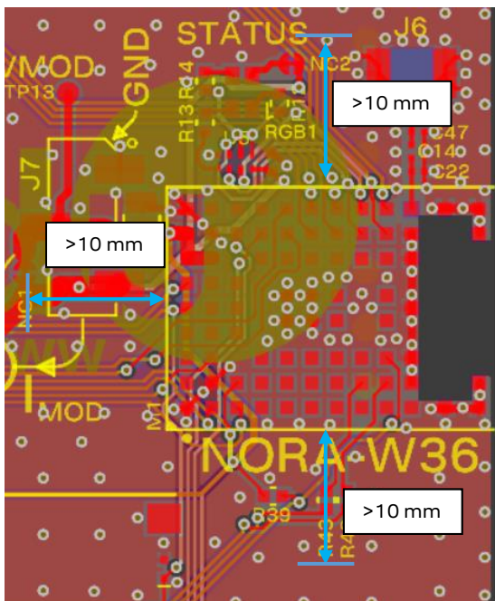
Figure 6: GND plane guard area enclosing NORA-W366
