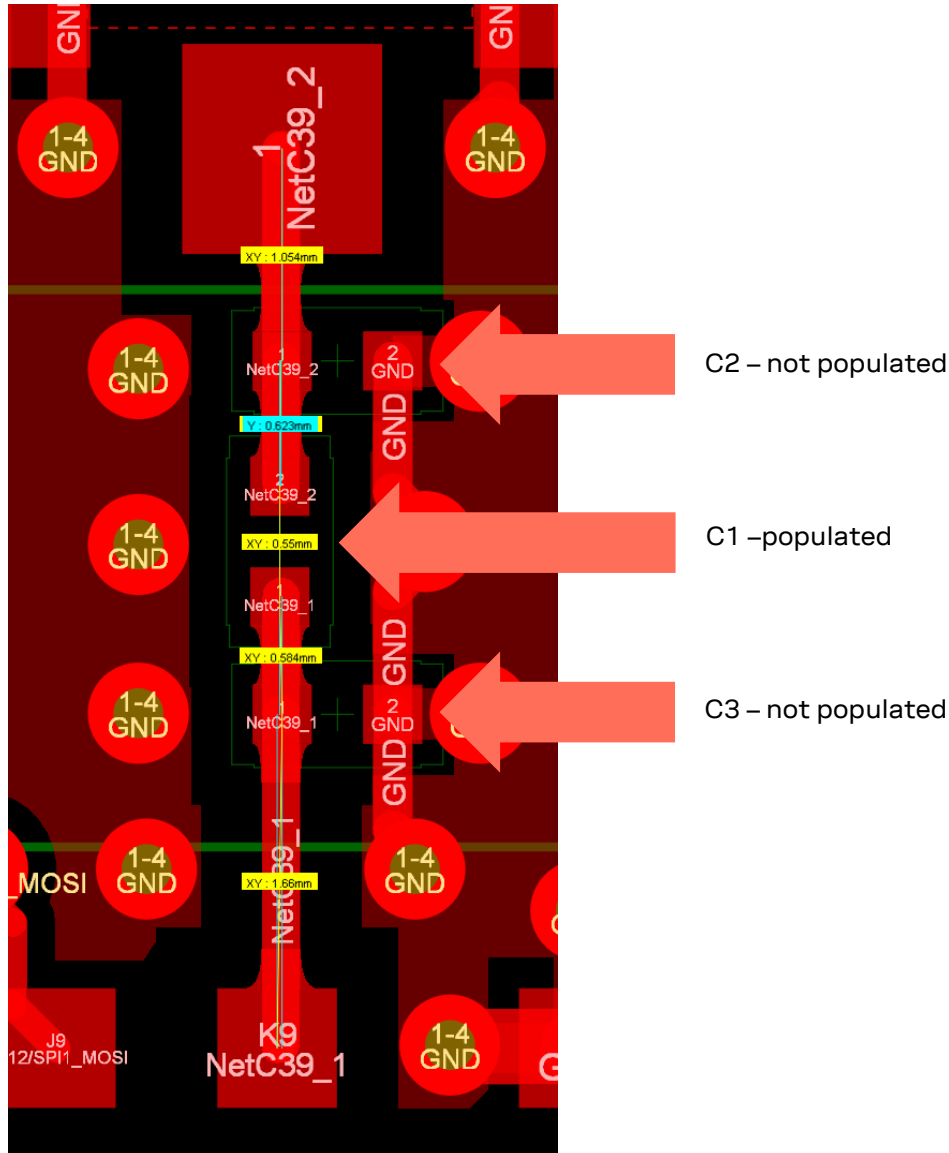
Figure 29: RF trace design component placement
