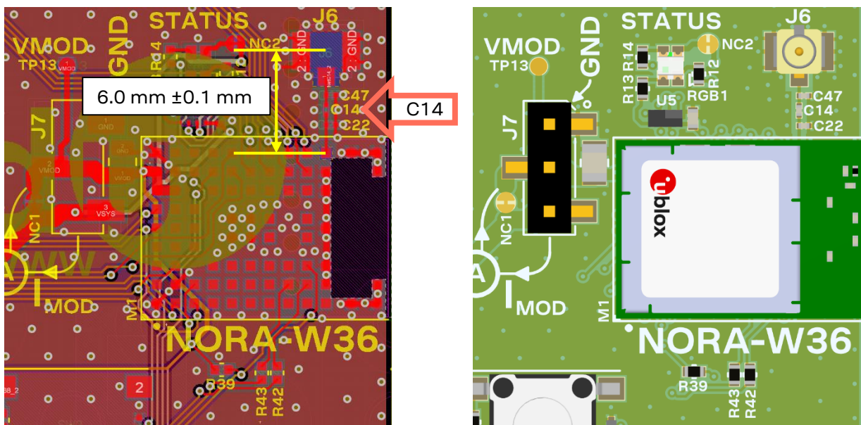
Figure 4: NORA-W361 approved U.FL antenna connection – 2D and 3D views
