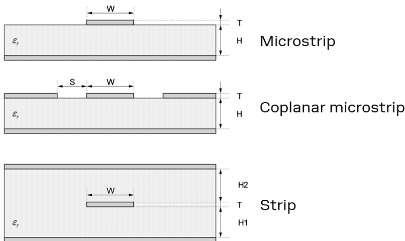
Figure 3: Transmission line trace design
