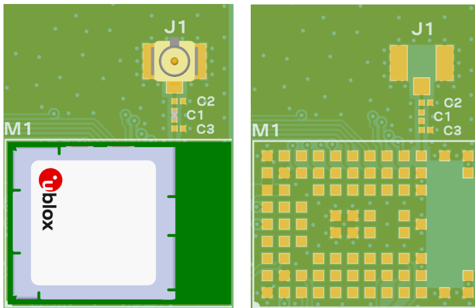
Figure 23: U.FL connector placement (left) and module footprint (right)
