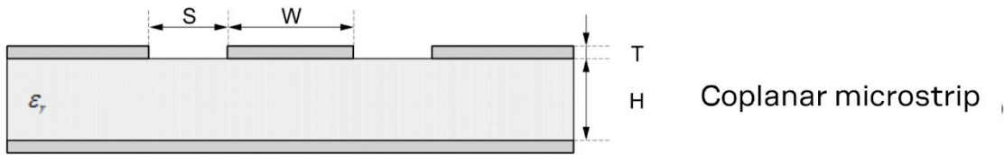
Figure 26: Coplanar micro-strip dimensions
