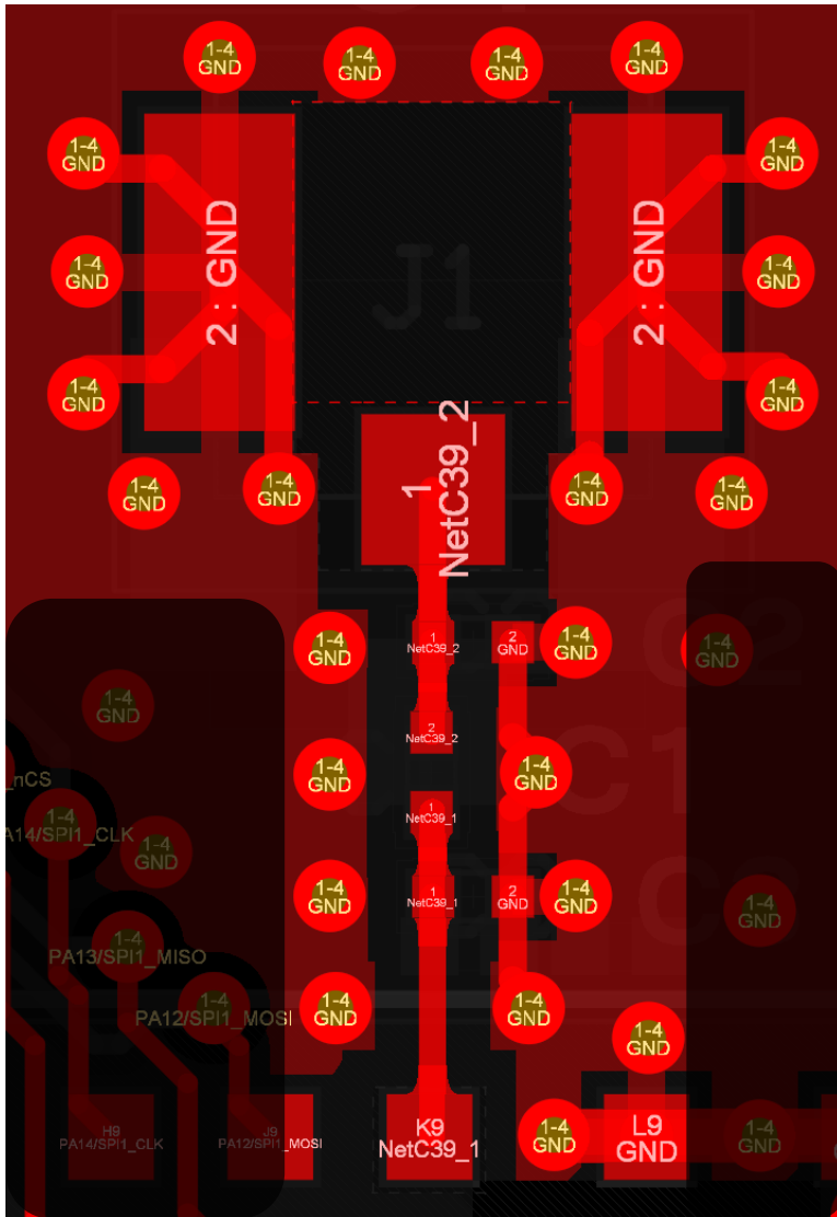
Figure 27: Layer 1 routing, keep-out, and ground stitching vias
