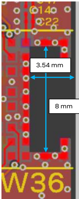
Figure 7: Size of the GND cut out for the NORA-W36 PCB trace antenna
