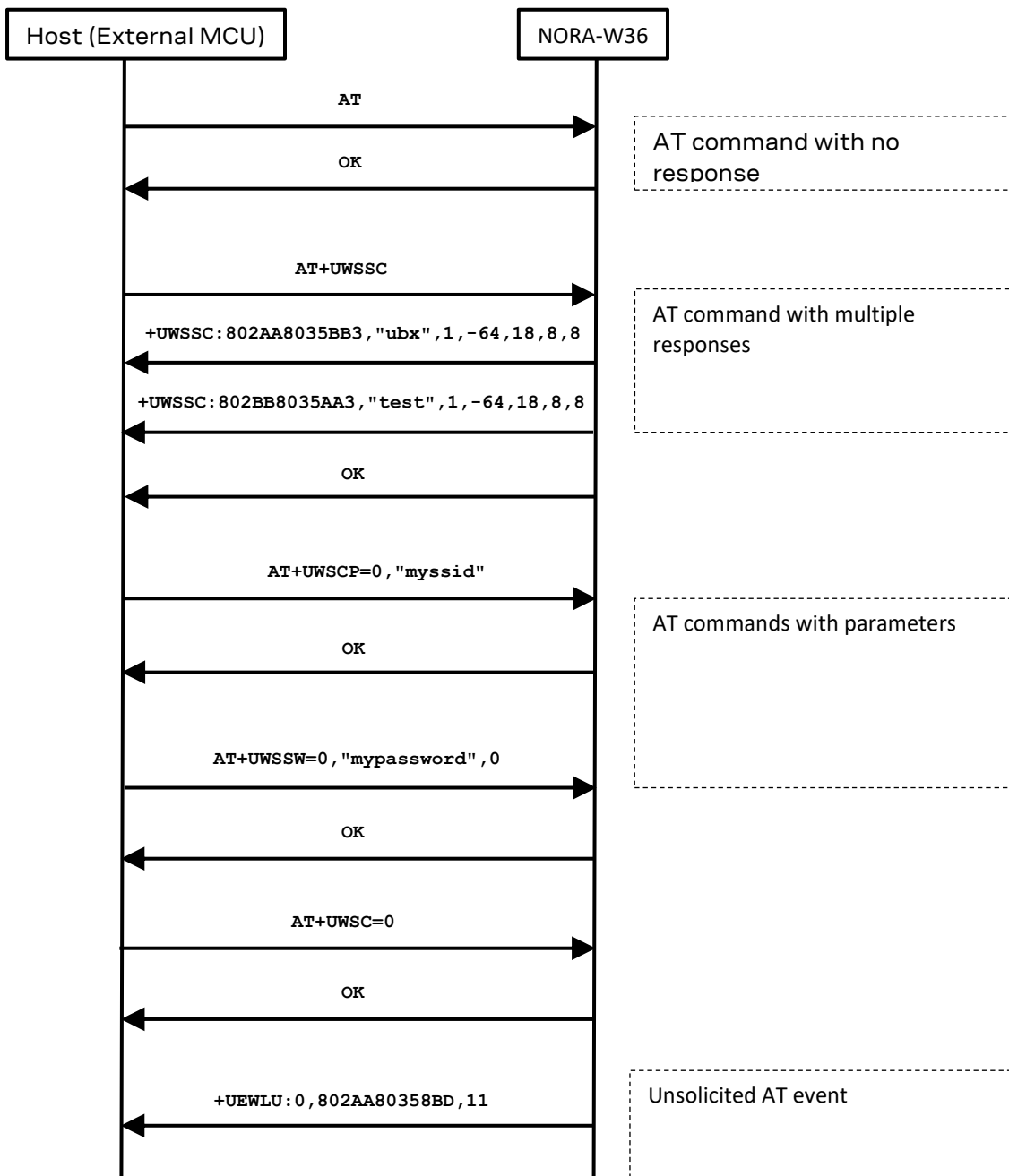
Figure 11: Example of AT commands and events
