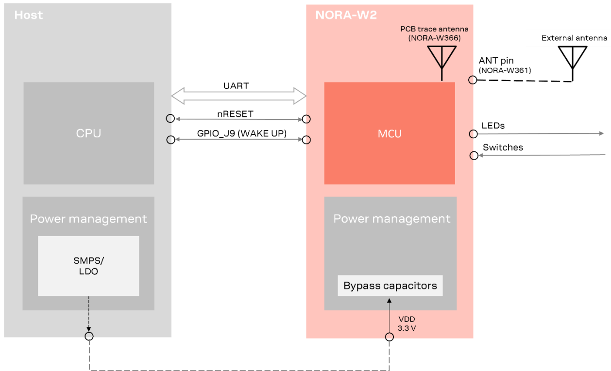
Figure 2: NORA-W36 integration in host system
