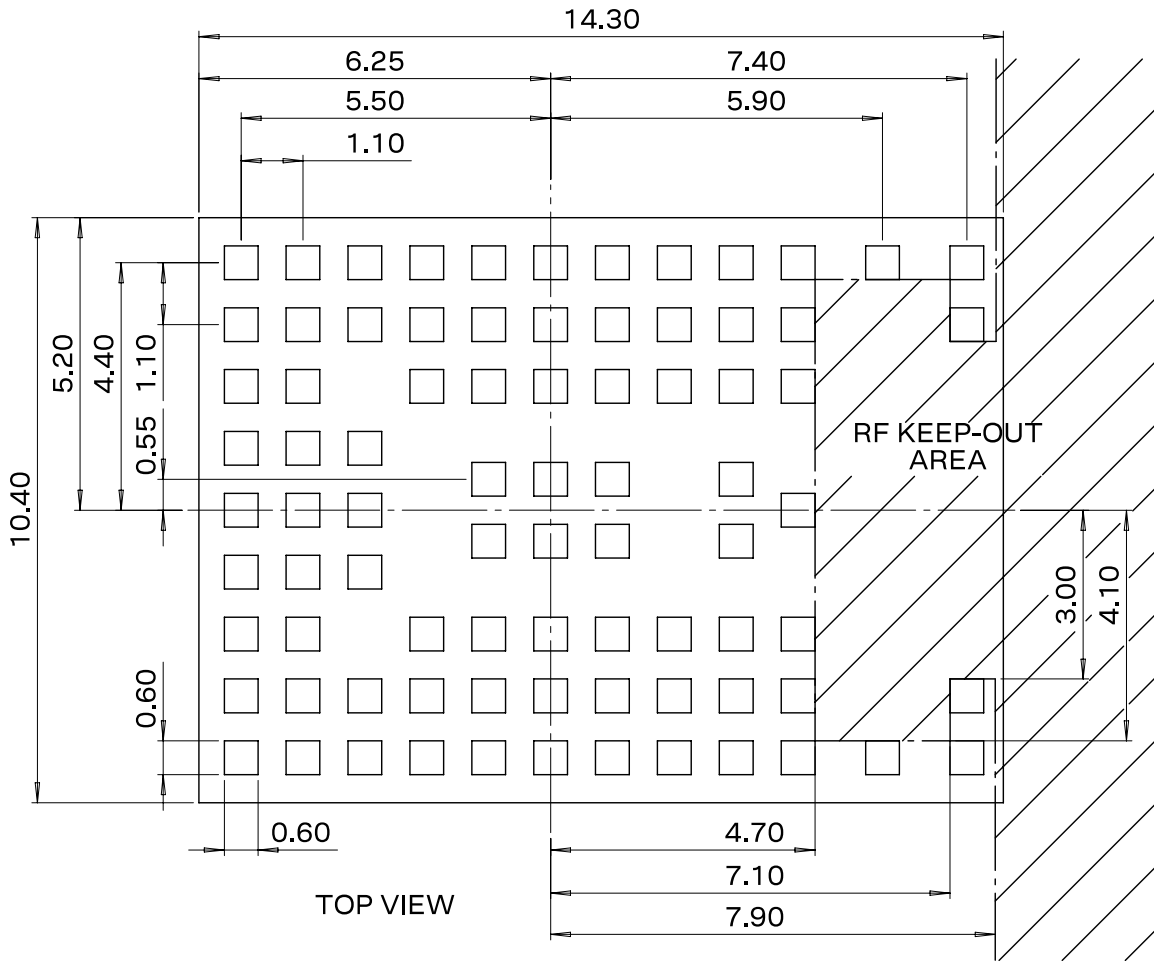
Figure 8: NORA-W36 mechanical outline
