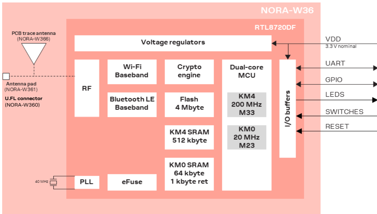
Figure 1: NORA-W36 series block diagram
