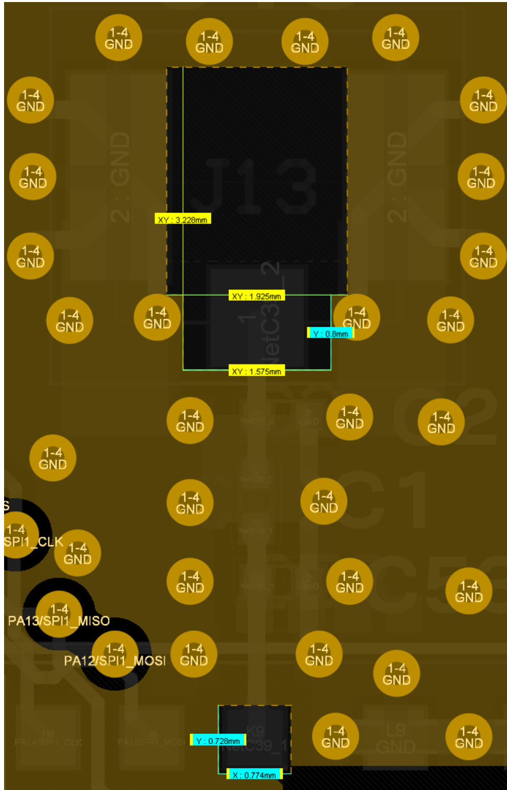
Figure 28: Layer 2 keep-out areas
