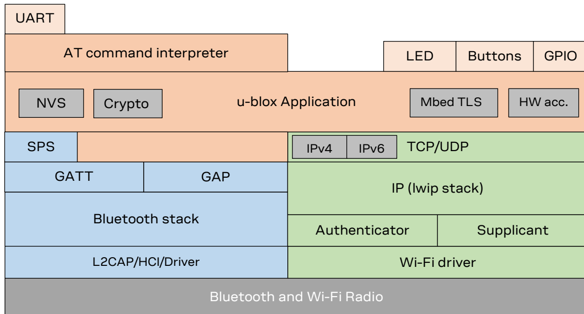
Figure 10: NORA-W36-connectXpress software architecture
