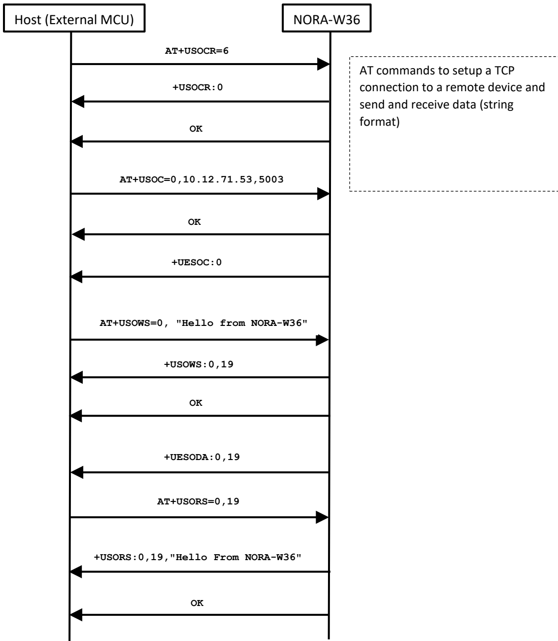
Figure 12: Example of AT command to setup TCP and send and receive data
