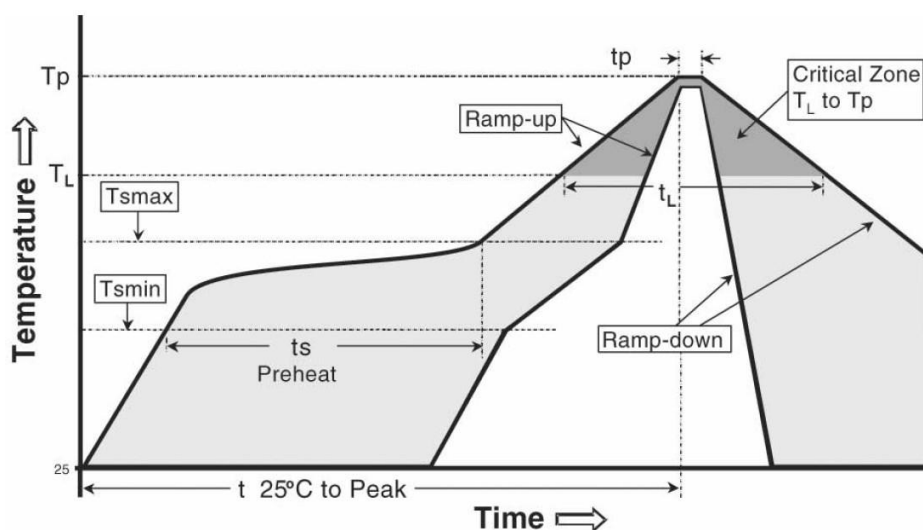
Figure 16: Reflow profile
