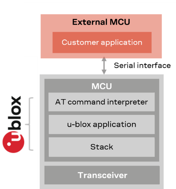
Figure 9: NORA-W36-connectXpress software structure
