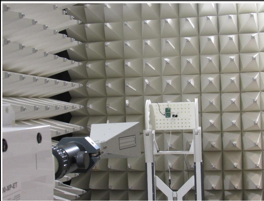
Setup above 1 GHz for Variant 2 (NORA-W101 with external antenna PN PRO-IS-237) -B
