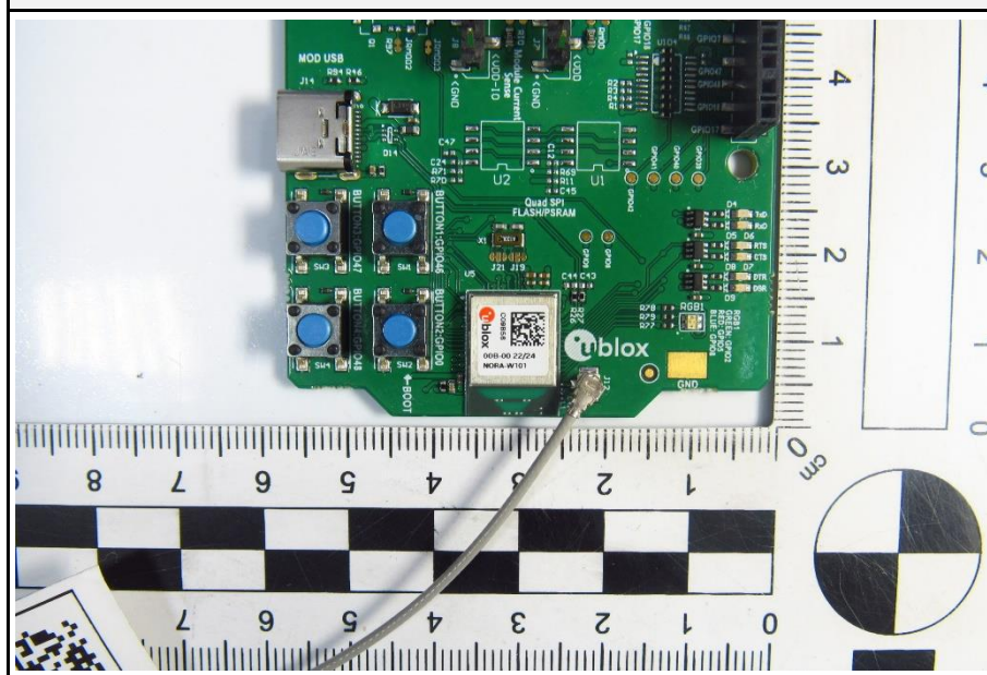
EUT radio module NORA-W101 view
