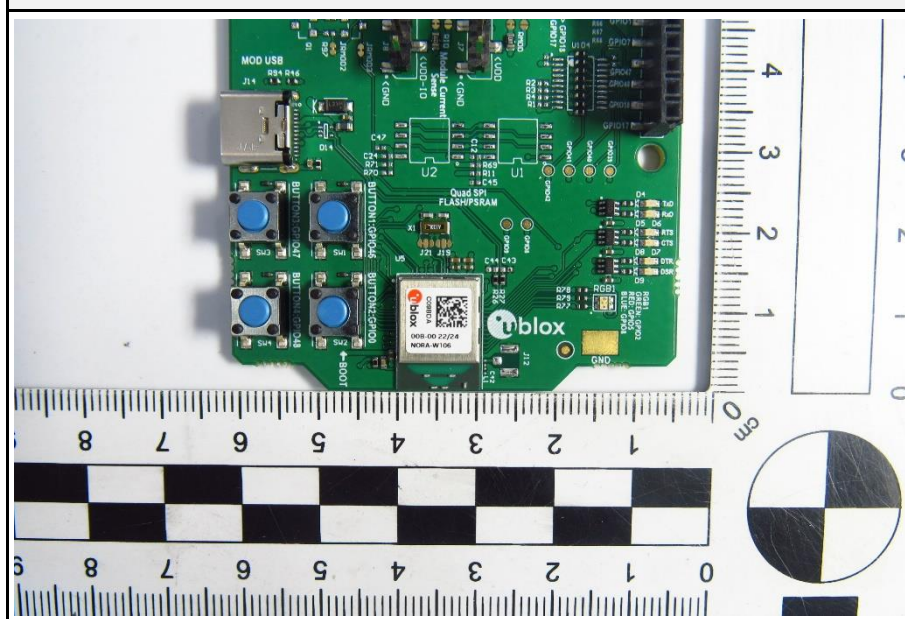
EUT radio module NORA-W106 view
