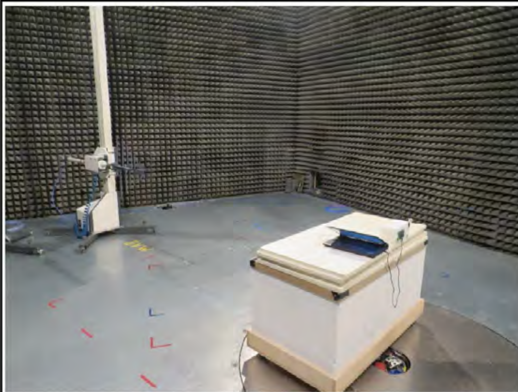
Setup below 1 GHz (NORA-W101) -B
