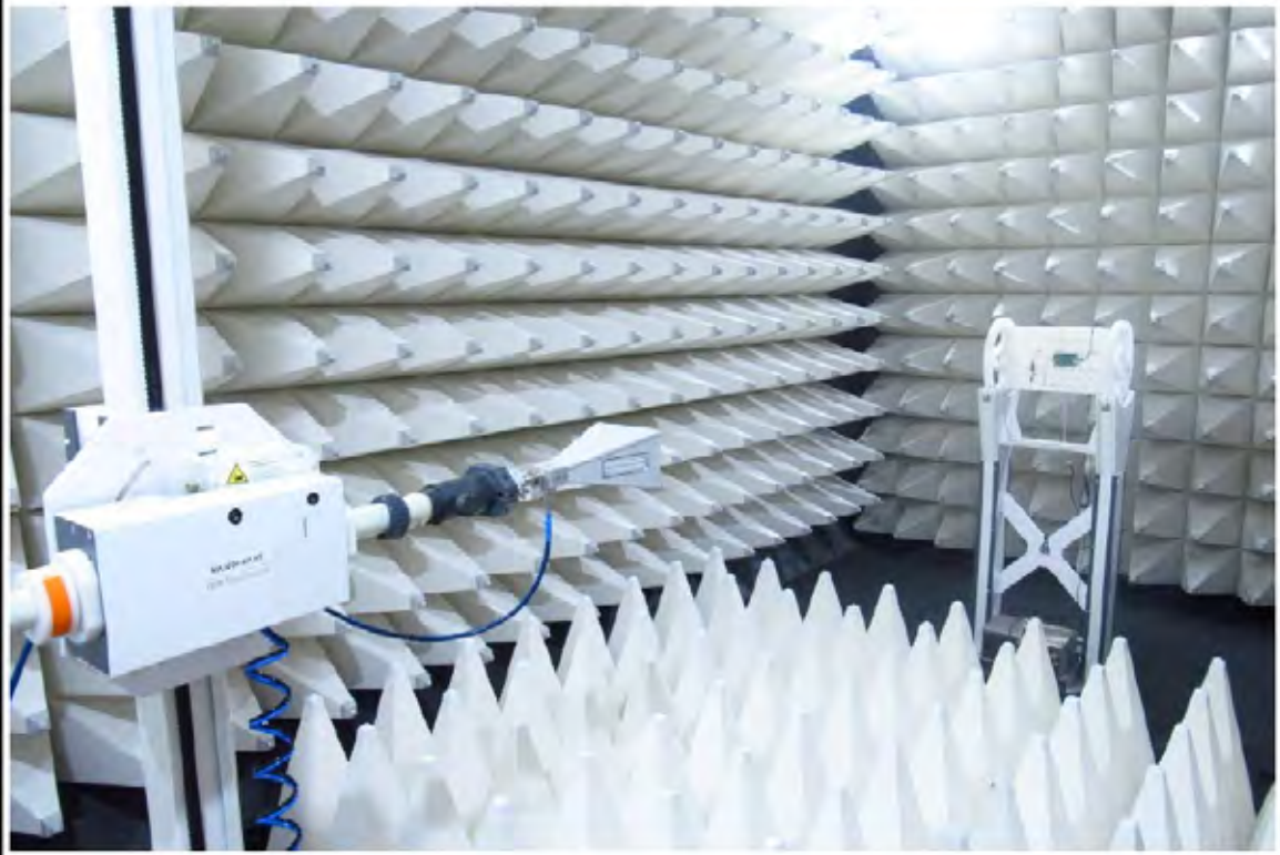
Setup above 1 GHz (NORA-W101) -A
