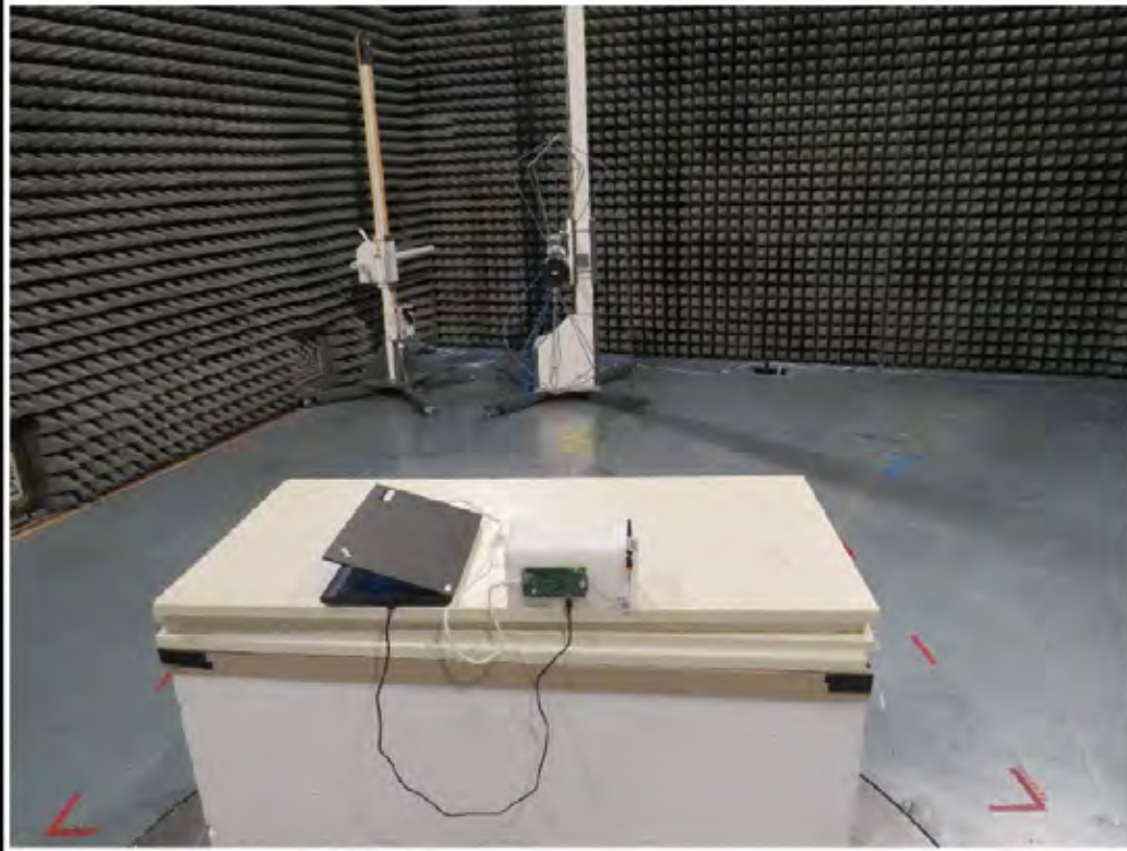
Setup below 1 GHz (NORA-W101) -A
