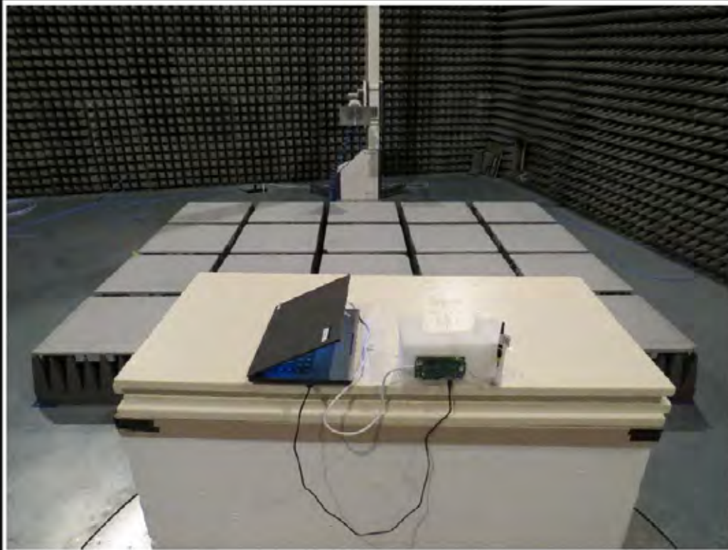
Setup above 1 GHz (NORA-W101)
