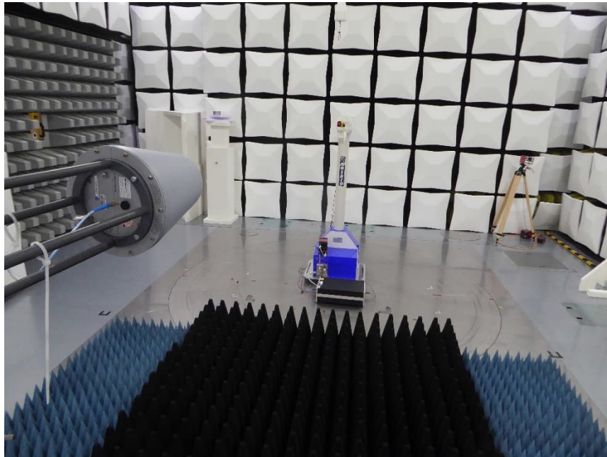
EUT on positioner Test setup fully anechoic chamber M276 Preliminary and final measurement 1 – 18 GHz
