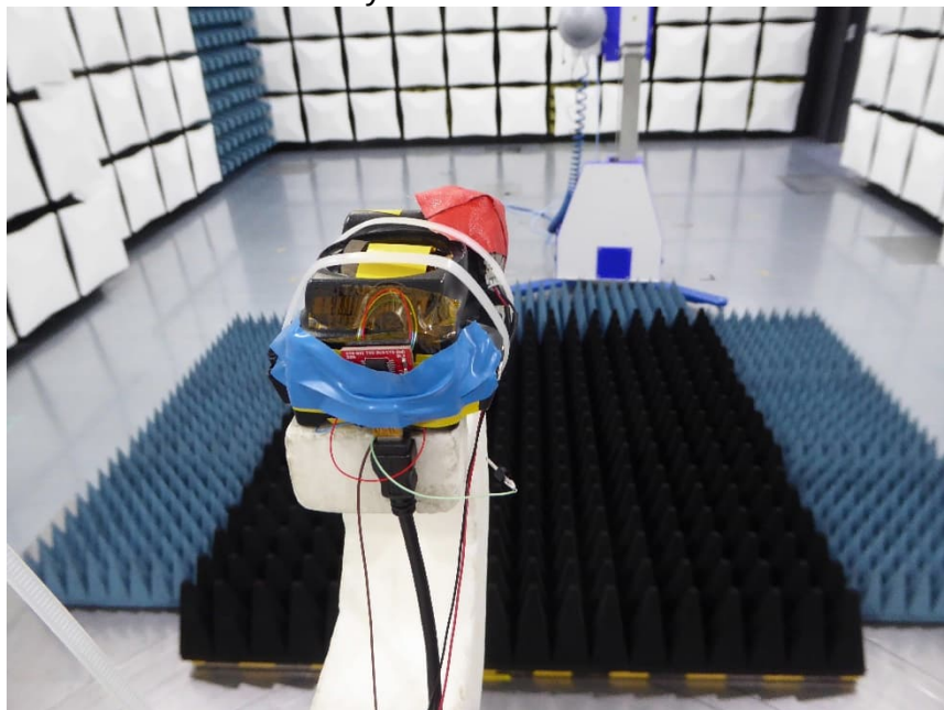
EUT on positioner Test setup fully anechoic chamber M276 Preliminary and final measurement
