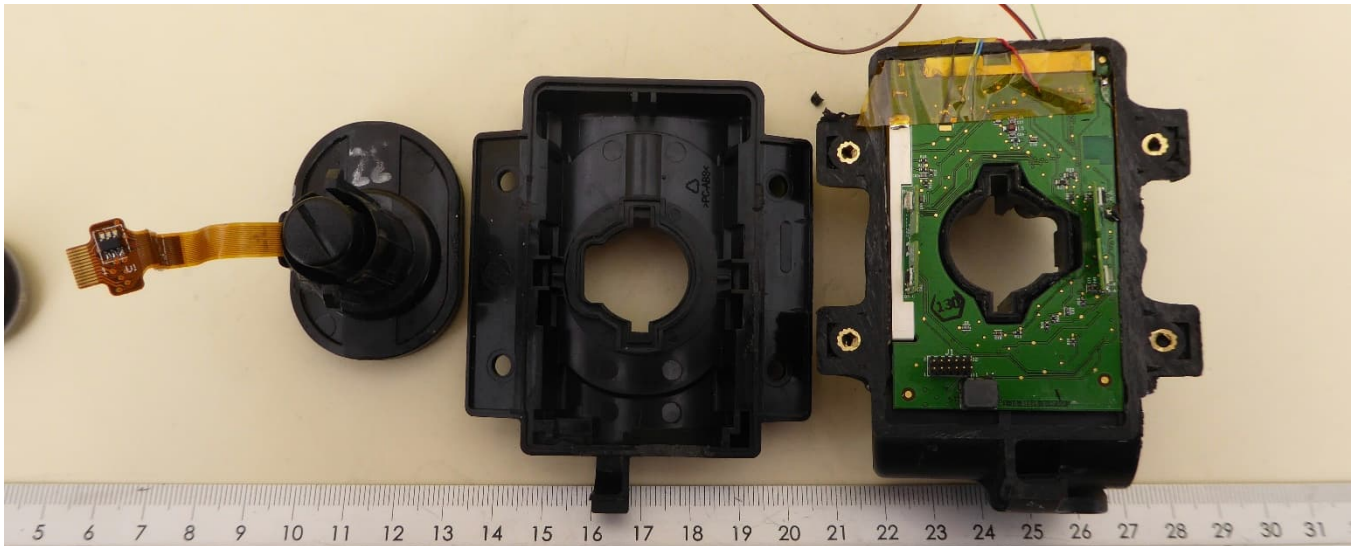
EUT opened
