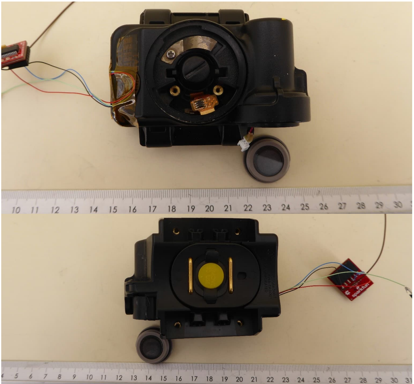
EUT external Top view & bottom view
