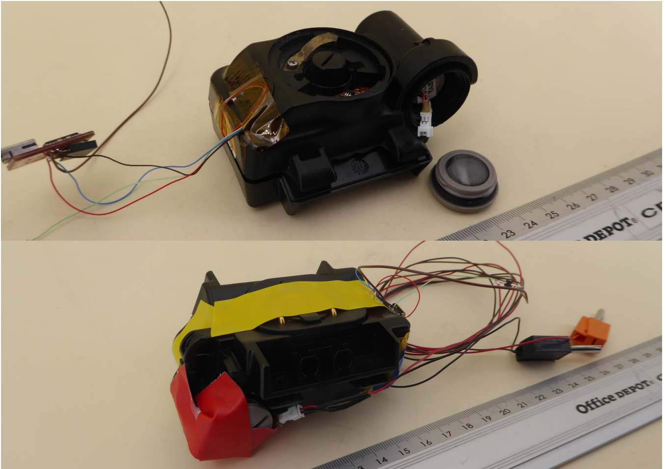
EUT external 3d top & 3d bottom view
