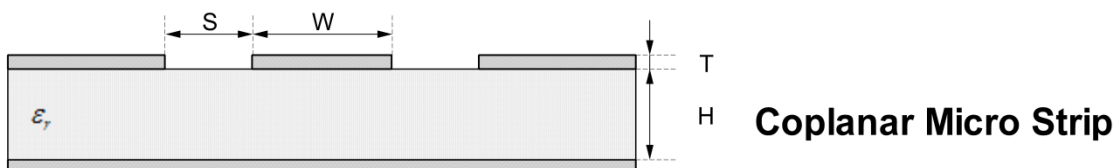
Figure 23: Coplanar micro-strip dimension specification
